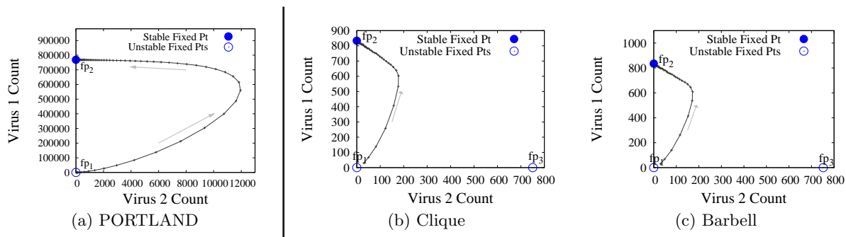
Figure 5: Phase plots (scatter plot of number of infected nodes by virus 2 and number of infected nodes by virus 1) plots for simulations on (a) the PORTLAND network, (b) a clique and (c) a barbell graph for scenario ABOVE. Again, stable fixed points are marked by bold circles and unstable fixed points by hollow circles ( FP_3 not shown in (a) for sake of clarity of the trajectory). The weaker virus tries to dominate (note the bulge), but it dies-out completely and the stronger virus wins, as our result predicted.
