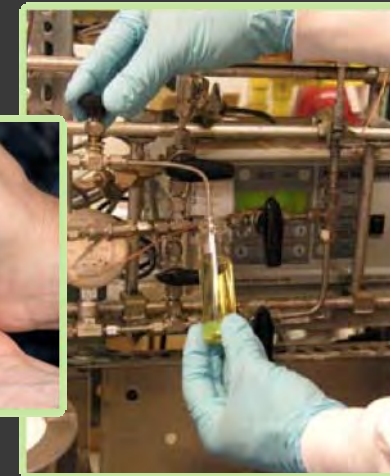
Coal-Biomass-to-Liquids
