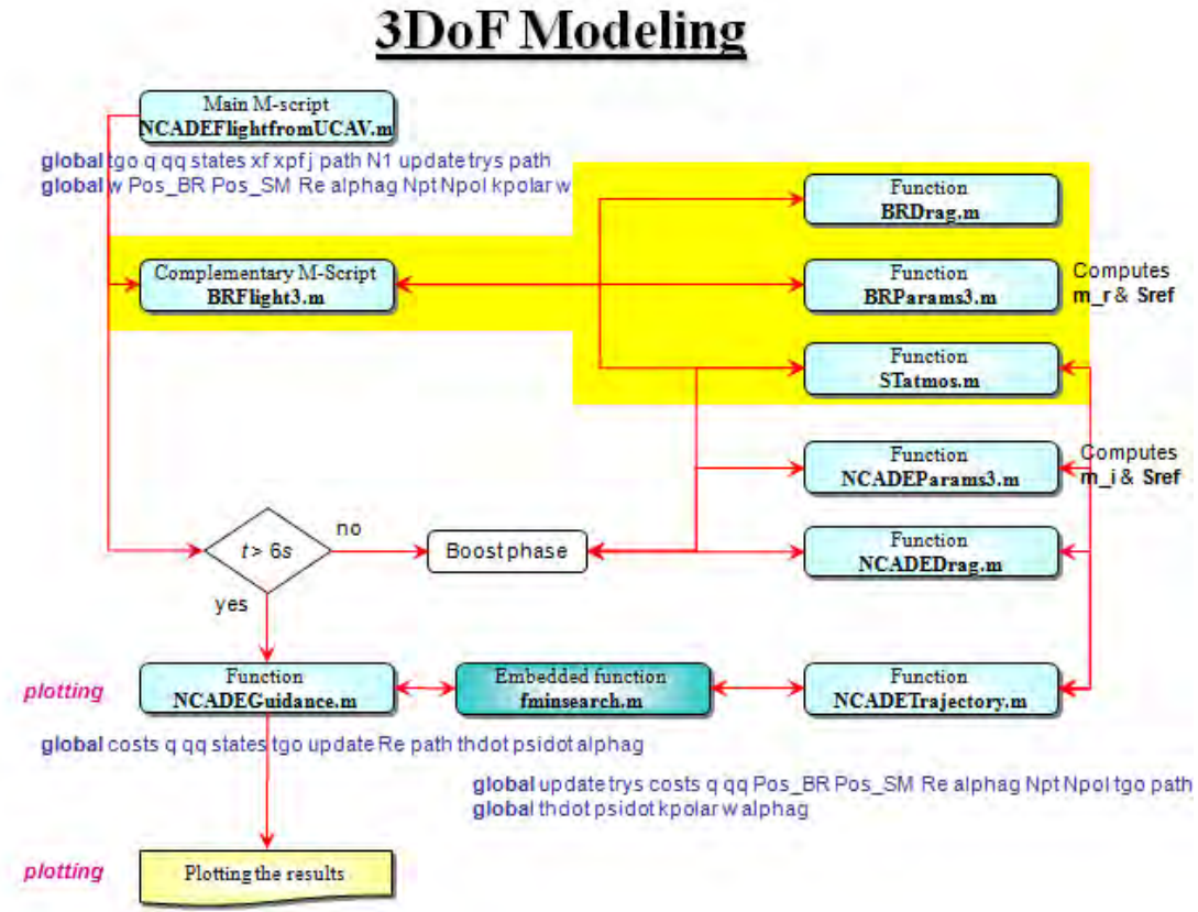
Figure 2. Simulation Flowchart
