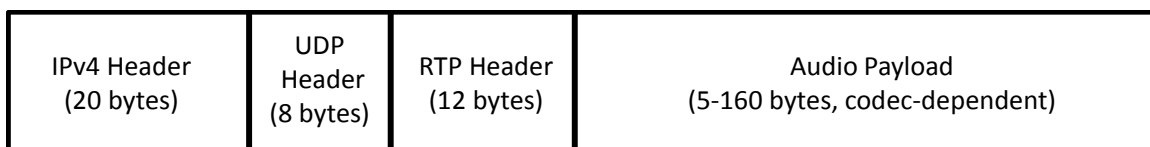
Figure 5: VoIP Packet Structure
