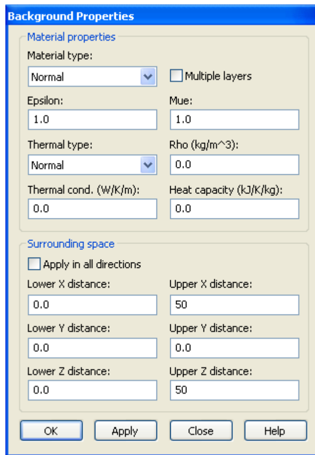
Figure 66. Setting for background properties (for coverage diagram test cases).
