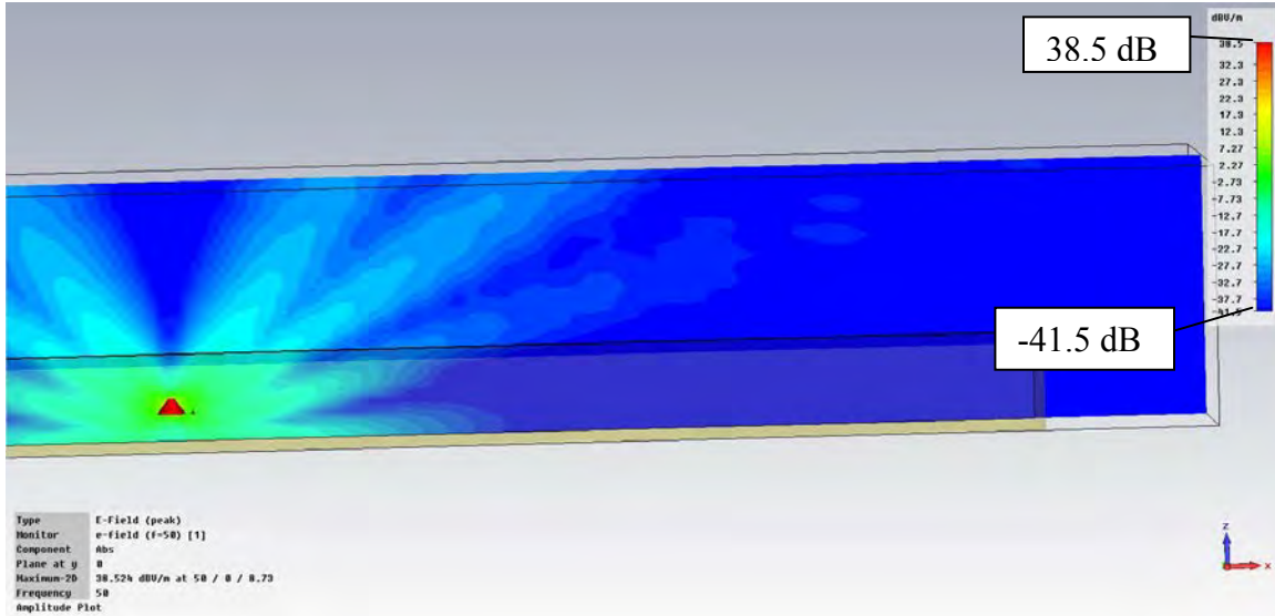
Figure 74. Coverage diagram for dipole antenna in foliage (height 10 m).
