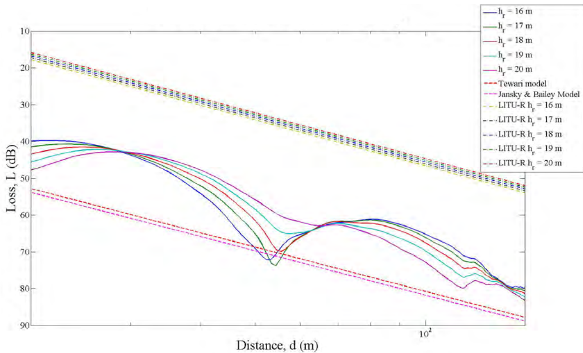
Figure 42. Loss-distance curves for h_r = 16-20 m (test case B3).
