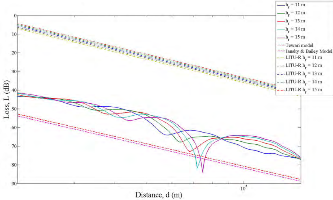
Figure 64. Loss–distance curves for h_r = 11–15 m (test case C5).
