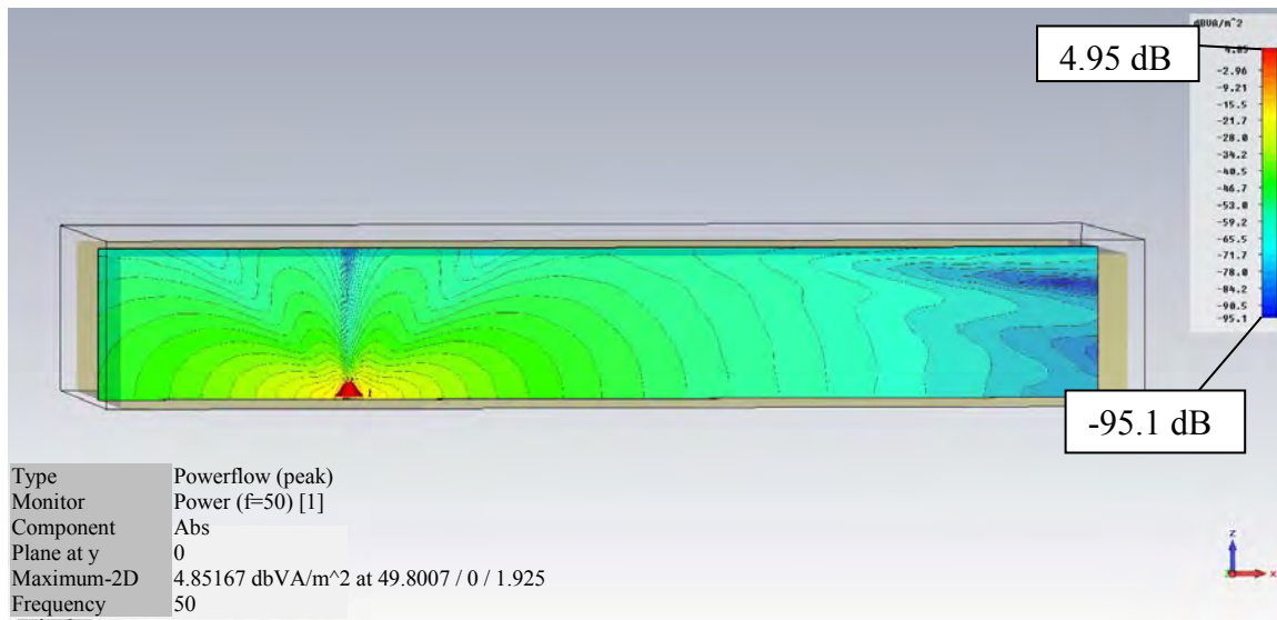
Figure 46. Power flow plot at y = 0 m for test case C1.
