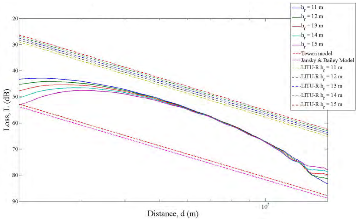
Figure 48. Loss-distance curves for h_r = 11-15 m (test case C1).
