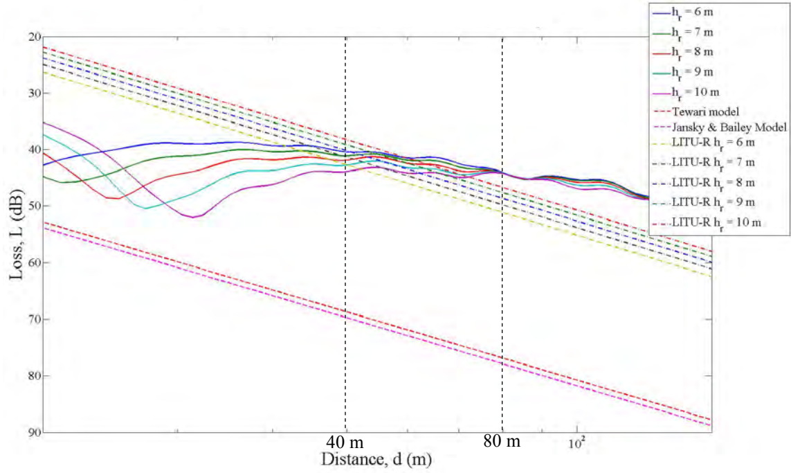
Figure 34. Loss–distance curves for h_r = 6\text{--}10 m (test case B1).
