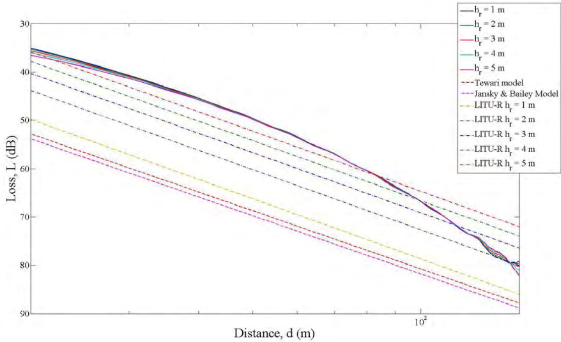
Figure 47. Loss-distance curves for h_r = 1-5 m (test case C1).
