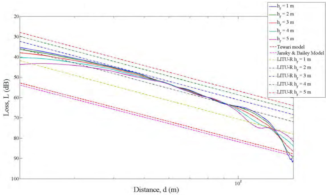
Figure 41. Loss-distance curves for h_r = 1-5 m (test case B3).
