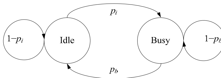
Figure 14. Two-state Markov model of primary user channel occupancy [5].
