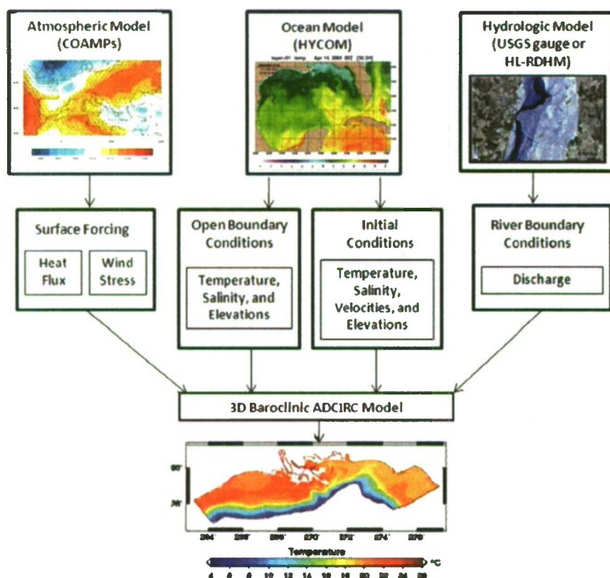
Fig. 15. Schematic of the coupled HYCOM-ADCIRC system.
