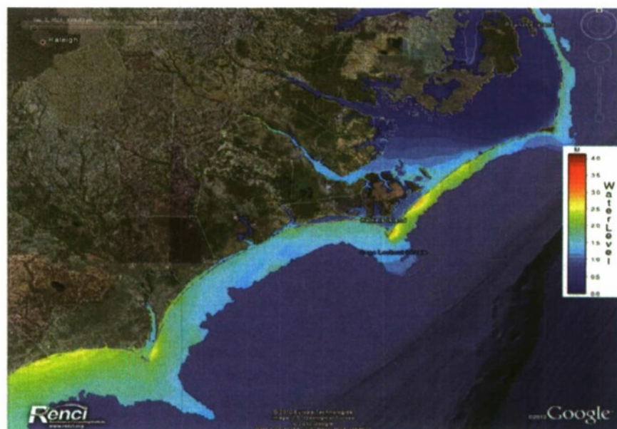
FIG. 13. Simulation of maximum inundation (m) for Hurricane Earl produced by CI-FLOW real-time system. Inundation calculated by subtracting surface elevations from total water level elevations, which account for freshwater flows from HL-RDHM and tides, waves, and surge from ADCIRC+SWAN.
