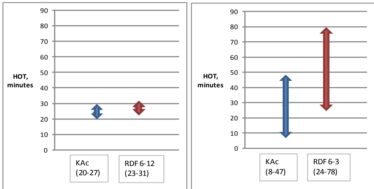
Figure 4. Comparison of Anti-Icing HOT Intervals for RDF 6-12 and RDF 6-3 versus KAc RDF
