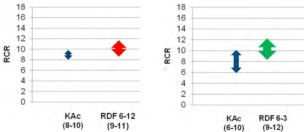
Figure 3. Comparison of Anti-Icing Friction Test Confidence Intervals for RDF 6-12 and RDF 6-3 versus KAc RDF
