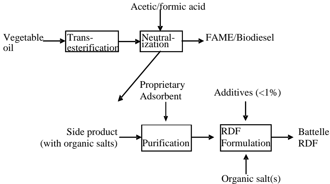
Figure 1. Battelle-RDF Process
