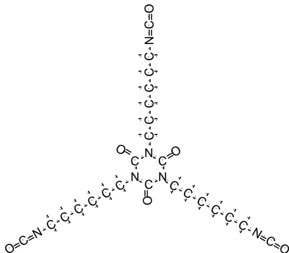
1,6-Hexamethylene Diisocyanate Crosslinker
