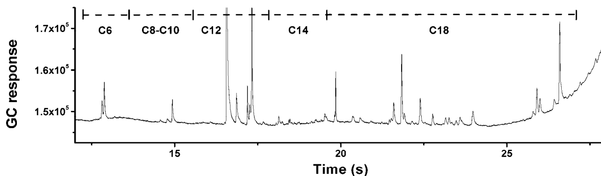
Figure 18. Typical gas chromatogram (FID detector, DB-17ms column), online technique. Adapted from Ref. 49.
