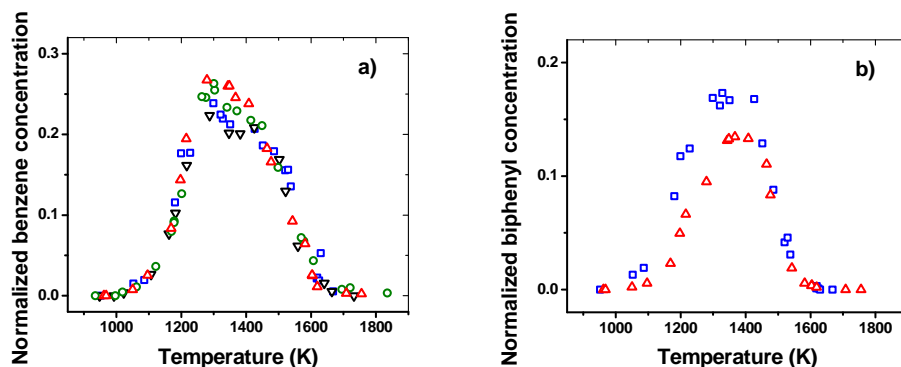
Figure 24. a) Normalized benzene decomposition; b) normalized biphenyl decomposition. \circ [C_6H_5I]_0 = 50.6 ppm, p \sim 50 atm; \Delta [C_6H_5I]_0 = 95.6 ppm, p \sim 50 atm; \square [C_6H_5I]_0 = 26.6 ppm, p \sim 50 atm; \nabla [C_6H_5I]_0 = 54.2 ppm, p \sim 25 atm.
