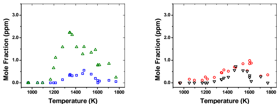
Figure 38. Experimental mole fraction, [C_6H_5I]_0 = 95.6 ppm, p \sim 50 atm. \Delta chrysene ( \sim 90\% ) + triphenylene ( \sim 10\% ); \square benzo[a]anthracene; \circ benzo[g,h,i]fluoranthene; \nabla benzo[c]phenanthrene.
