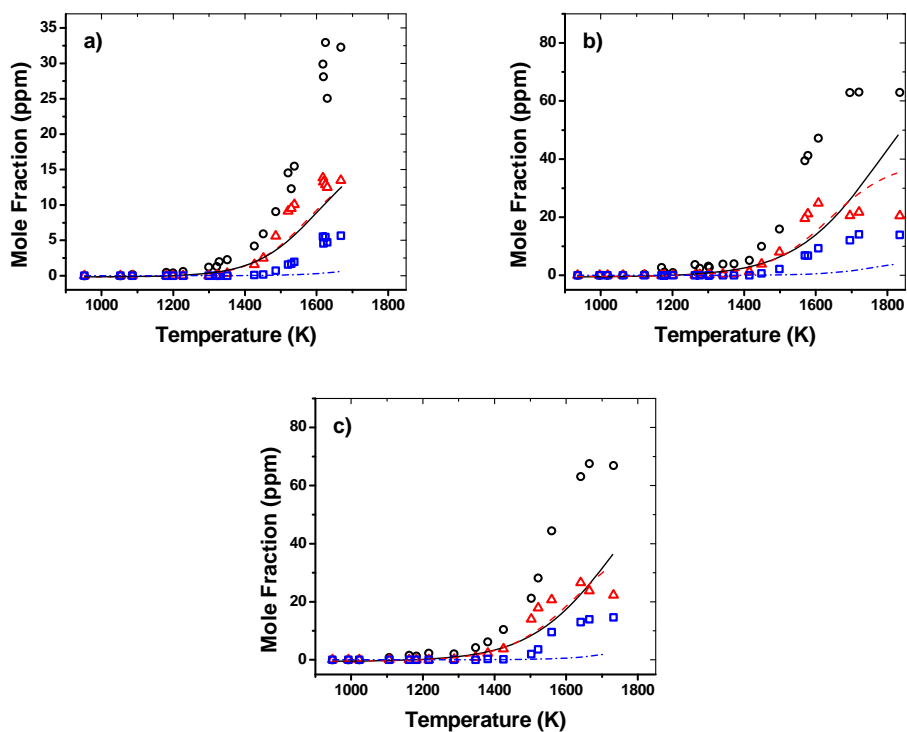
Figure 42. \circ Acetylene exp., — acetylene sim.; \Delta diacetylene exp., - - diacetylene sim.; \square triacetylene exp., - \cdot - triacetylene sim. a) [C_6H_5I]_0 = 26.6 ppm, p \sim 50 atm; b) [C_6H_5I]_0 = 50.6 ppm, p \sim 50 atm; c) [C_6H_5I]_0 = 54.2 ppm, p \sim 25 atm.
