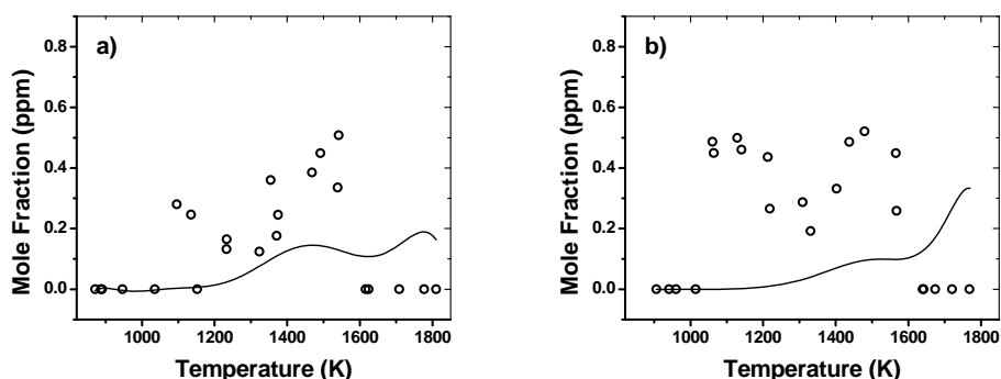
Figure 52. \circ Naphthalene exp., — naphthalene sim. a) [C_6H_5I]_0 = 58.1 ppm, [C_2H_2]_0 = 236.3 ppm, p \sim 50 atm; b) [C_6H_5I]_0 = 55.1 ppm, [C_2H_2]_0 = 511.3 ppm, p \sim 50 atm.
