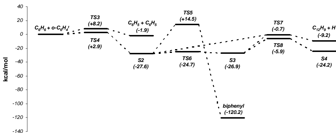
Figure 61. Potential energy surface for benzene + triplet o-benzyne radical/ \pi -bond addition. uCCSD(T)/cc-pVDZ relative energies in kcal/mol, including ZPVE.
