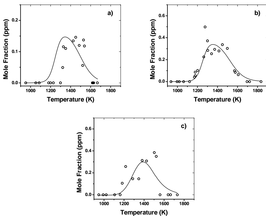
Figure 37. \circ Naphthalene exp., — naphthalene sim. a) [C_6H_5I]_0 = 26.6 ppm, p \sim 50 atm; b) [C_6H_5I]_0 = 50.6 ppm, p \sim 50 atm; c) [C_6H_5I]_0 = 54.2 ppm, p \sim 25 atm.
