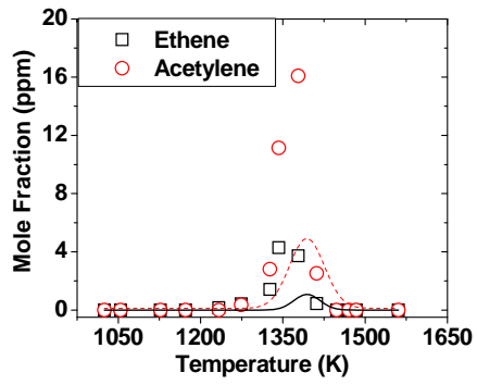
Figure 104. Comparison of experimental and modeling profiles for m-xylene oxidation, average P5 = 27 atm, \Phi = 0.55 , nominal reaction time = 1.5 ms, [□]- Experiments, [-]-UIC m-Xylene Model 2.
