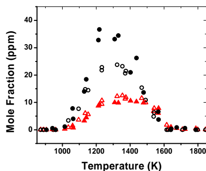
Figure 46. Experiments, p \sim 50 atm. \circ phenylacetylene, [C_6H_5I]_0 = 58.1 ppm, [C_2H_2]_0 = 236.3 ppm; \triangle benzene, [C_6H_5I]_0 = 58.1 ppm, [C_2H_2]_0 = 236.3 ppm; \bullet phenylacetylene, [C_6H_5I]_0 = 55.1 ppm, [C_2H_2]_0 = 511.3 ppm; \blacktriangle benzene, [C_6H_5I]_0 = 55.1 ppm, [C_2H_2]_0 = 511.3 ppm.
