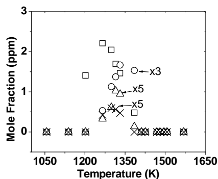
Figure 86. m-Xylene oxidation species profiles, average P5 = 53 atm, \Phi = 0.53 , nominal reaction time = 1.5 ms [\square] -3,3'-Dimethylbibenzyl, [o] -di-m-Tolylmethane, [\Delta] -m-Tolyl-p-tolylmethane, [X] -Bibenzyl.
