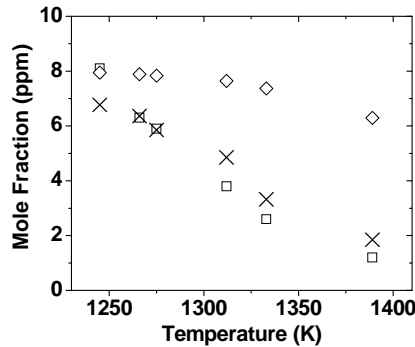
Figure 96. Comparison of the toluene oxidation experimental data and the modeling results [24], average P5 = 543 atm, \Phi = 1 , nominal reaction time = 1.4 ms, \square - Experiments, \diamond - Updated Toluene Oxidation Model 2, \times -Updated Toluene Oxidation Model 3.
