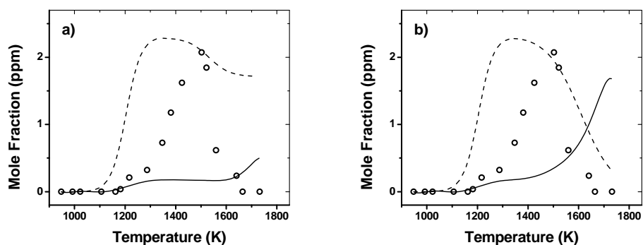
Figure 34. \circ Acenaphthylene exp.; — acenaphthylene sim.; -- cyclopenta[a]indene sim. a) model in Table 8 omitting reaction R80; b) model in Table 8 with k_{80} calculated from [83]. [\text{C}_6\text{H}_5\text{I}]_0 = 54.2\text{ ppm} , p \sim 25\text{ atm} .
