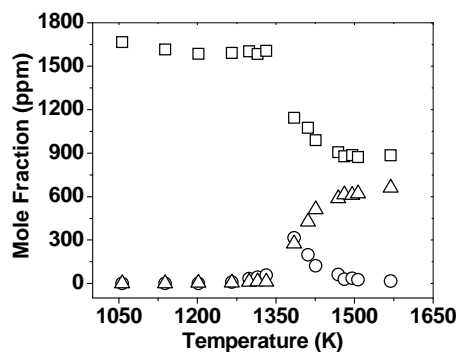
Figure 84. m-Xylene oxidation species profiles, average P5 = 53 atm, \Phi = 0.53 , nominal reaction time = 1.5 ms, [□]-O 2 , [○]-CO, [△]-CO 2 .
