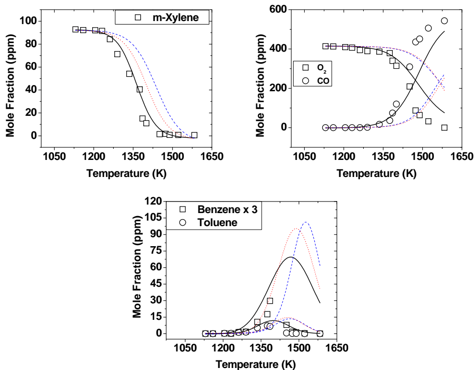
Figure 93. Comparison of experimental and modeling profiles for m-xylene oxidation, average P5 = 51 atm, \Phi = 2.35 , nominal reaction time = 1.5 ms, [□]- Experiments, [-]-Battin-Leclerc et al. model [29], [...]-Gail and Dagaut model [28], [---]-Narayanaswamy et al. model [144].
