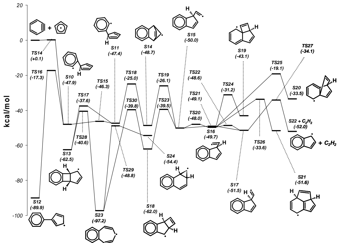
Figure 80. Potential energy surface for the radical/π-bond addition between o-benzyne and cyclopentadienyl radical. uB3LYP/6-311+G(d,p) relative energies in kcal/mol, including ZPVE.
