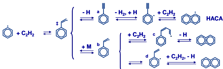
Figure 2. Formation of naphthalene from phenyl + acetylene reaction.
