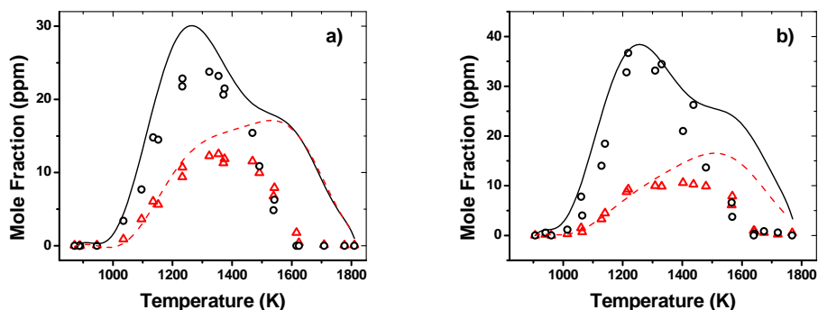
Figure 48. \circ Phenylacetylene exp., — phenylacetylene sim.; \Delta benzene exp., -- benzene sim. a) [C_6H_5I]_0 = 58.1 ppm, [C_2H_2]_0 = 236.3 ppm, p \sim 50 atm; b) [C_6H_5I]_0 = 55.1 ppm, [C_2H_2]_0 = 511.3 ppm, p \sim 50 atm.
