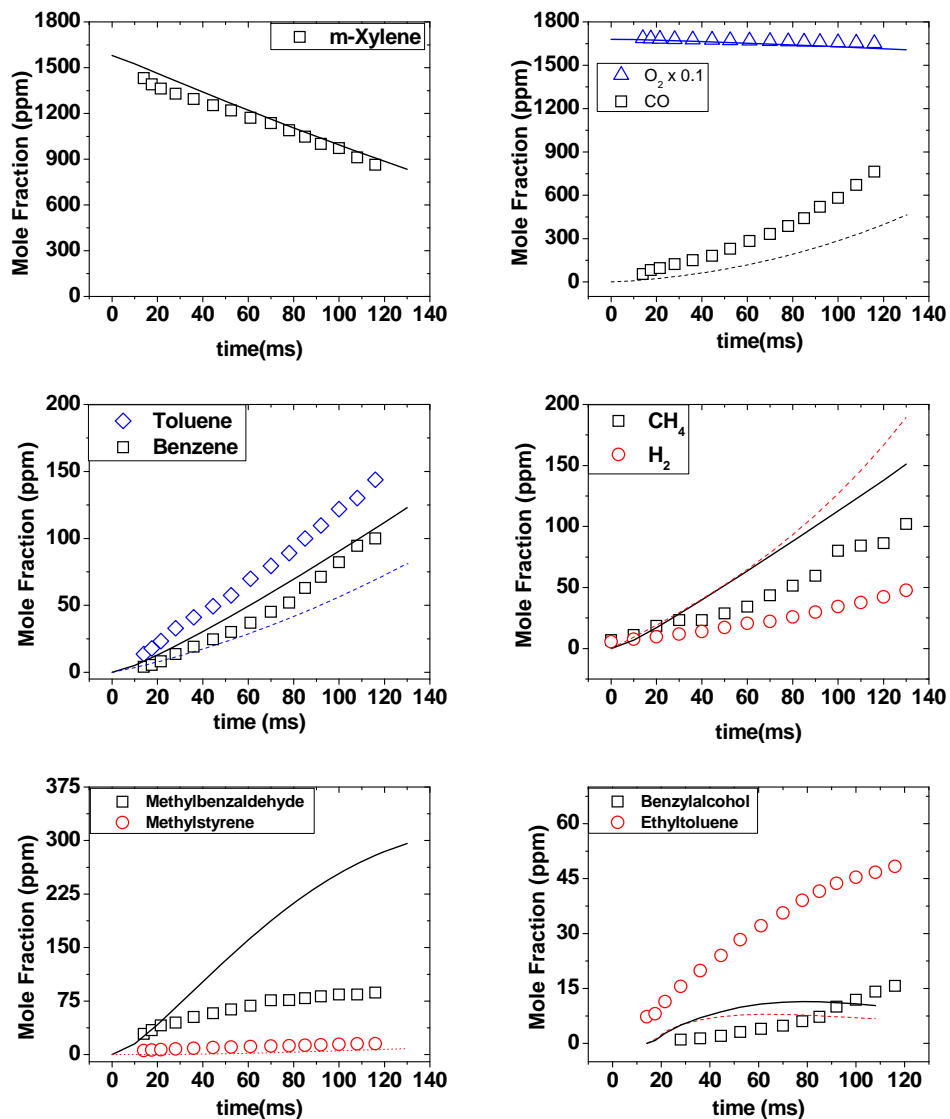
Figure 107. m-Xylene oxidation flow reactor experiments at atmospheric pressure, Emdee et al. [27] time shift = 10 ms, comparison of experimental and modeling predictions \square - Experiments, [-]-UIC m-Xylene Model 2
