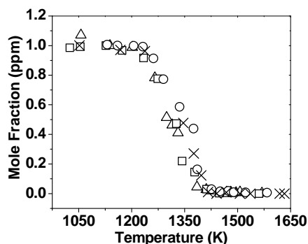
Figure 83. m-Xylene decay, [▲]-average P5 = 53 atm, \Phi = 0.53 , [◻]-average P5 = 27 atm, \Phi = 0.55 , [○]-average P5 = 50 atm, \Phi = 2.35 , [×]- average P5 = 28 atm, \Phi = 2.1 , nominal reaction time = 1.5 ms.
