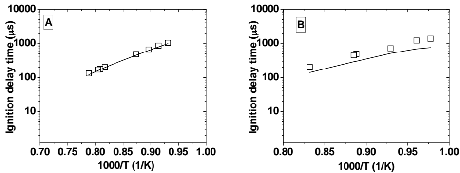
Figure 103. m-Xylene/air, P = 45 atm, (A) \Phi = 0.5 , (B) \Phi = 1 , comparison of experimental ignition delay data of Shen and Oehlschlaeger [30] and modeling results, [□]- Experiments, [-]-UIC m-Xylene Model 2.
