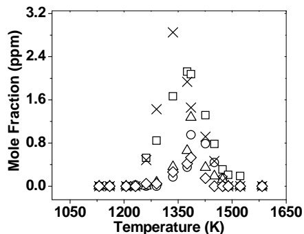
Figure 89. m-Xylene oxidation species profiles, average P5 = 50 atm, \Phi = 2.35 , nominal reaction time = 1.5 ms, [□]-Naphthalene, [ \Delta ]-Anthracene, [X]-Indene, [o]-Acenaphthylene, [◇]-Fluorene.
