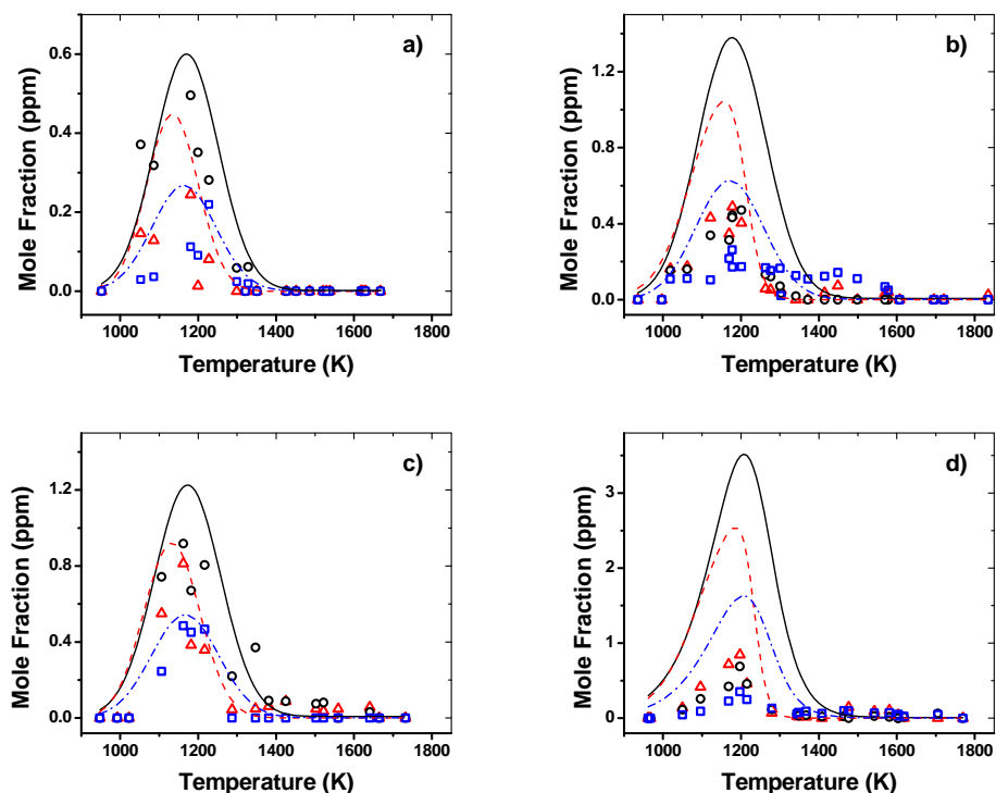
Figure 29. \Delta o-Iodobiphenyl exp., -- o-iodobiphenyl sim.; \circ m-iodobiphenyl exp., — m-iodobiphenyl sim.; \square p-iodobiphenyl exp., - · - p-iodobiphenyl sim. a) [C_6H_5I]_0 = 26.6 ppm, p \sim 50 atm; b) [C_6H_5I]_0 = 50.6 ppm, p \sim 50 atm; c) [C_6H_5I]_0 = 54.2 ppm, p \sim 25 atm; d) [C_6H_5I]_0 = 95.6 ppm, p \sim 50 atm.
