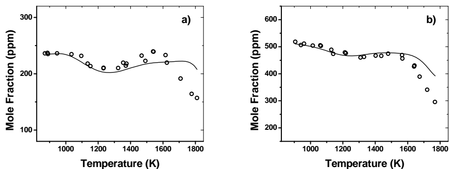
Figure 45. Acetylene decomposition. \circ exp.; — sim. a) [C_6H_5I]_0 = 58.1 ppm, [C_2H_2]_0 = 236.3 ppm, p \sim 50 atm; b) [C_6H_5I]_0 = 55.1 ppm, [C_2H_2]_0 = 511.3 ppm, p \sim 50 atm.
