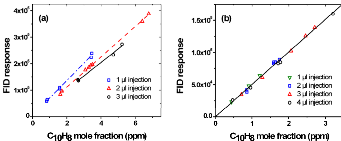
Figure 10. FID gas calibrations. A) 10 \mu\text{l} syringe; B) 5 \mu\text{l} syringe with plunger in the needle.
