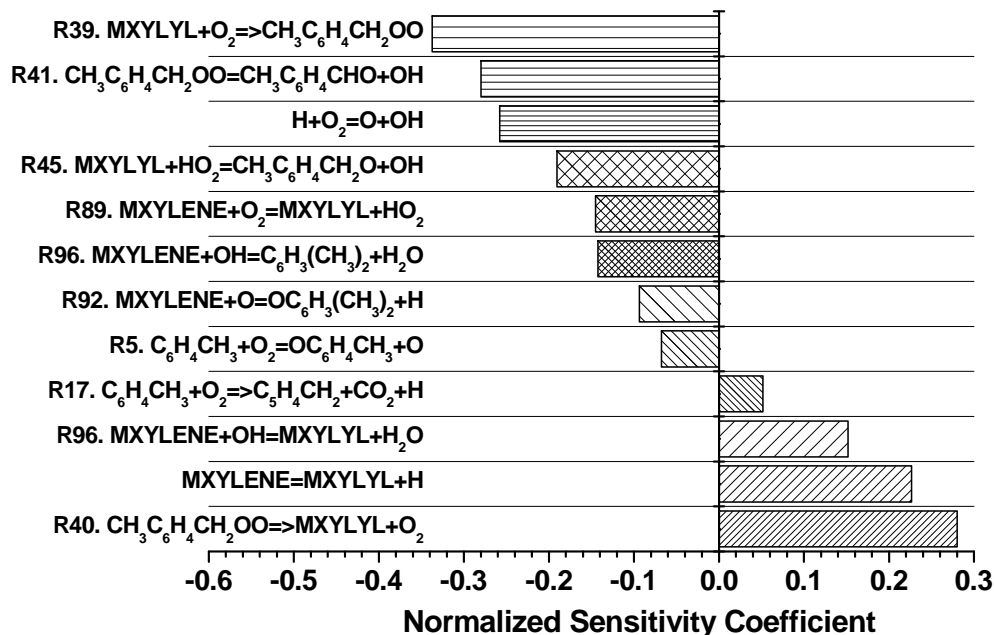
Figure 111. Sensitivity analysis of m-xylene performed for T = 1161 K, P = 1 atm and time = 0.1s, using UIC m-Xylene Oxidation Model 2.
