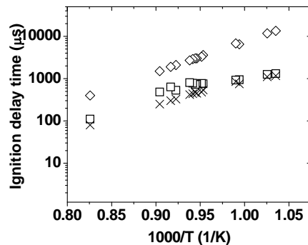
Figure 97. Toluene/air, P5 = 50 atm, \Phi = 1 , comparison of the experimental data [147] and the modeling results, \square - Experiments, \diamond -Updated Toluene Oxidation Model 2, \times -Updated Toluene Oxidation Model 3.
