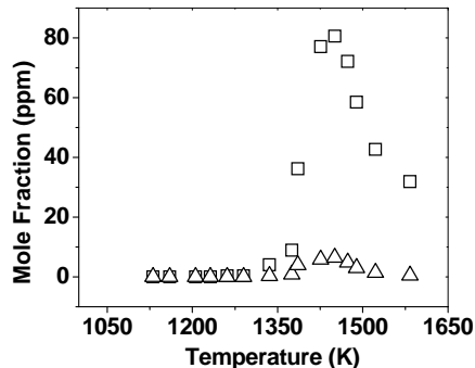
Figure 91. m-Xylene oxidation, species profiles, average P5 = 50 atm, \Phi = 2.35 , nominal reaction time = 1.5 ms, [□]- Acetylene, [△]-Diacetylene.
