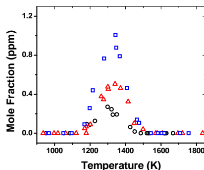
Figure 31. Biphenylene experimental concentrations at p \sim 50 atm. \circ [C_6H_5I]_0 = 26.6 ppm; \triangle [C_6H_5I]_0 = 50.6 ppm; \square [C_6H_5I]_0 = 95.6 ppm.
