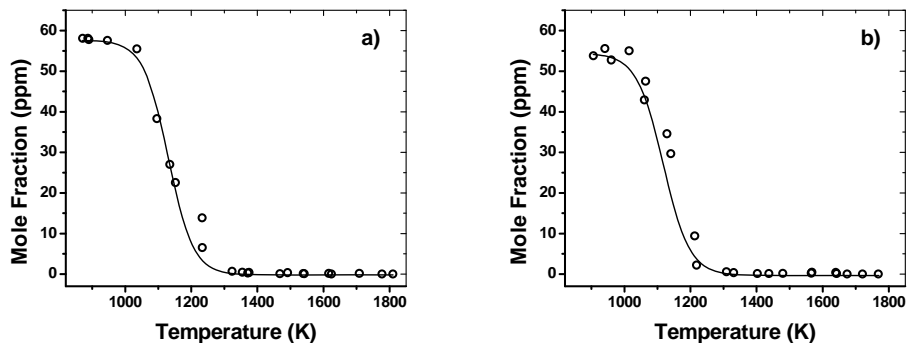
Figure 44. Phenyl iodide decomposition. \circ exp.; — sim. a) [C_6H_5I]_0 = 58.1 ppm, [C_2H_2]_0 = 236.3 ppm, p \sim 50 atm; b) [C_6H_5I]_0 = 55.1 ppm, [C_2H_2]_0 = 511.3 ppm, p \sim 50 atm.
