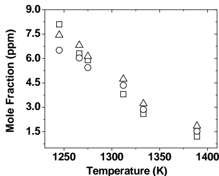
Figure 94. Comparison of the experimental data and the modeling results for toluene oxidation [24], average P_5 = 543 atm, \Phi = 1 , nominal reaction time = 1.4 ms, [□]- Experiments, [Δ]-High Pressure Toluene Oxidation Model [24], [○]-Updated Toluene Oxidation Model 1.
