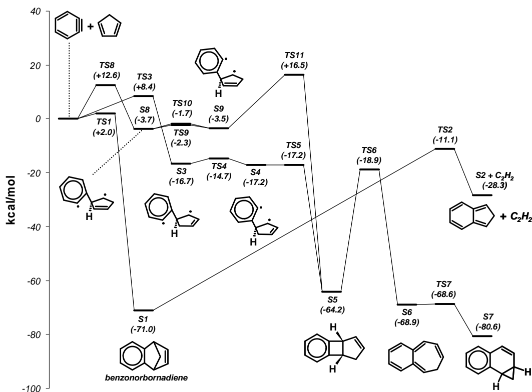
Figure 74. Potential energy surface for the radical/π-bond addition between o -benzyne and cyclopentadiene. uB3LYP/6-311+G(d,p) relative energies in kcal/mol, including ZPVE.
