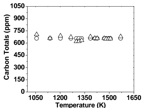
Figure 87. m-Xylene oxidation carbon totals, average P5 = 53 atm, nominal reaction time = 1.5 ms, \Phi = 0.53 , [o]-Preshock carbon, [ \Delta ]-Postshock carbon.
