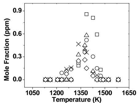
Figure 90. m-Xylene oxidation species profiles, average P5 = 50 atm, \Phi = 2.35 , nominal reaction time = 1.5 ms, [□]-1-Methylindene [ \Delta ]-1-Methylnaphthalene, [X]- 1,3,6-Trimethylnaphthalene, [o]-2-Methylantracene, [◇]-2-Methylphenanthrene.
