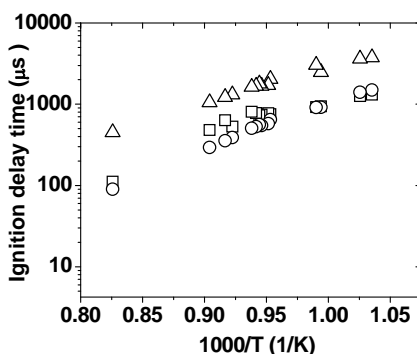
Figure 95. Toluene/air, P_5 = 50 atm, \Phi = 1 , comparison of experimental ignition delay data of S.S. Vasu et al. [147] and modeling results, [□]- Experiments, [Δ]-High Pressure Toluene Oxidation Model [24], [○]-Updated Toluene Oxidation Model 1.
