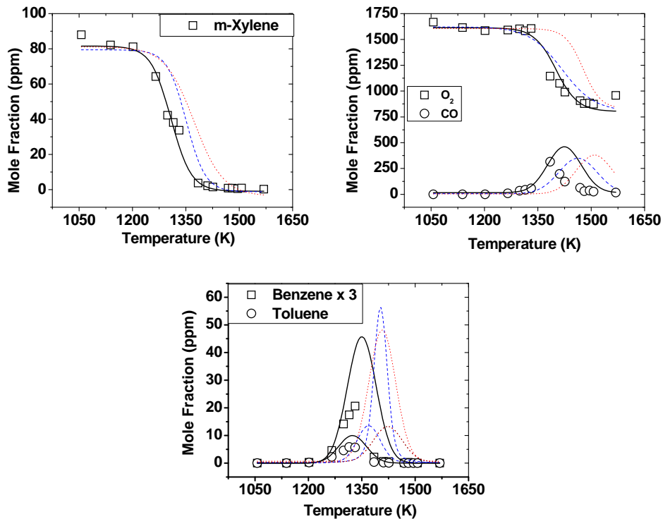
Figure 92. Comparison of experimental and modeling profiles for m-xylene oxidation, average P_5 = 53 atm, \Phi = 0.53 , nominal reaction time = 1.5 ms, [□]-Experiments, [-]-Battin-Leclerc et al. model [29], [...]-Gail and Dagaut model [28], [---]-Narayanaswamy et al. model [144].
