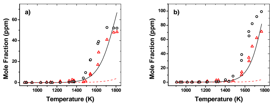
Figure 54. \circ Diacetylene exp., — diacetylene sim.; \Delta triacetylene exp., -- triacetylene sim. a) [C_6H_5I]_0 = 58.1 ppm, [C_2H_2]_0 = 236.3 ppm, p \sim 50 atm; b) [C_6H_5I]_0 = 55.1 ppm, [C_2H_2]_0 = 511.3 ppm, p \sim 50 atm.
