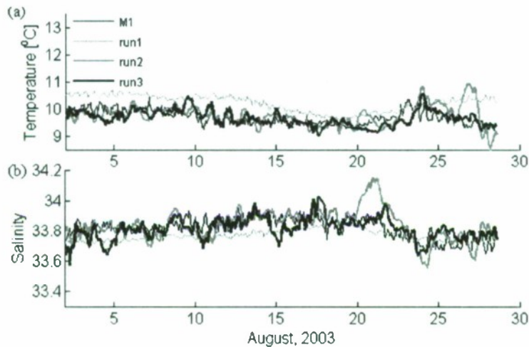
Figure 4. Temperature comparisons between results of run 1, run 2, run 3 and M1 observations at 60 m depth (a). Salinity comparisons between run 1, run 2, and run 3 and M1 observations at 60 m depth (b).
