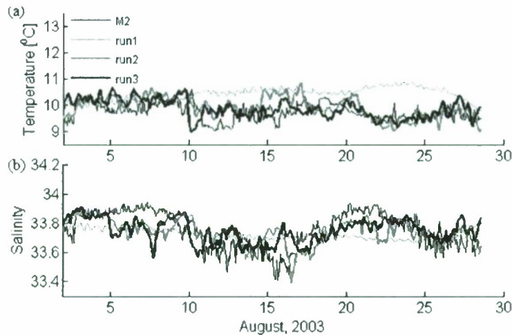
Figure 5. Temperature comparisons between results of run 1, run 2, run 3 and M2 observations at 60 m depth (a). Salinity comparisons between run 1, run 2, and run 3 and M2 observations at 60 m depth (b).
