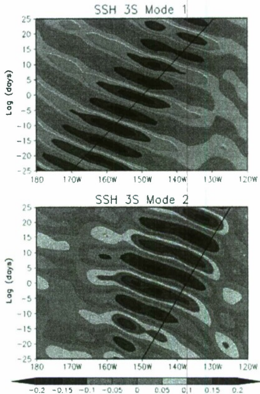
Figure 4. Upper panel: longitude–time diagram of regressed sea-surface-height anomalies for the first baroclinic mode. The solid line indicates the group velocity ( 1.03\text{ m s}^{-1} ) for the first baroclinic mode Yanai wave at the wavenumber 4007\text{ km} (the global wave number -10 for the horizontal axis in Figure 1) derived from the dispersion curve in Figure 1. Lower panel: same as the upper panel except for the second baroclinic mode of which the group velocity is 0.64\text{ m s}^{-1} .
