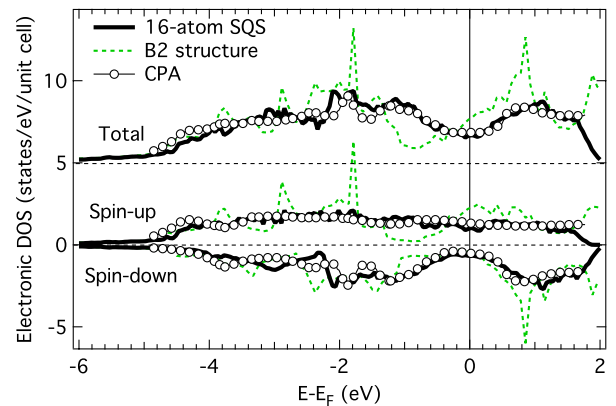
FIG. 3 (color online). Spin-polarized electronic DOS computed from first-principles with VASP for equiatomic FeV in the B2 structure, and in a 16-atom SQS. Calculations performed by Johnson et al. [29] using a CPA method are included for comparison. The total eDOS is offset for clarity.
