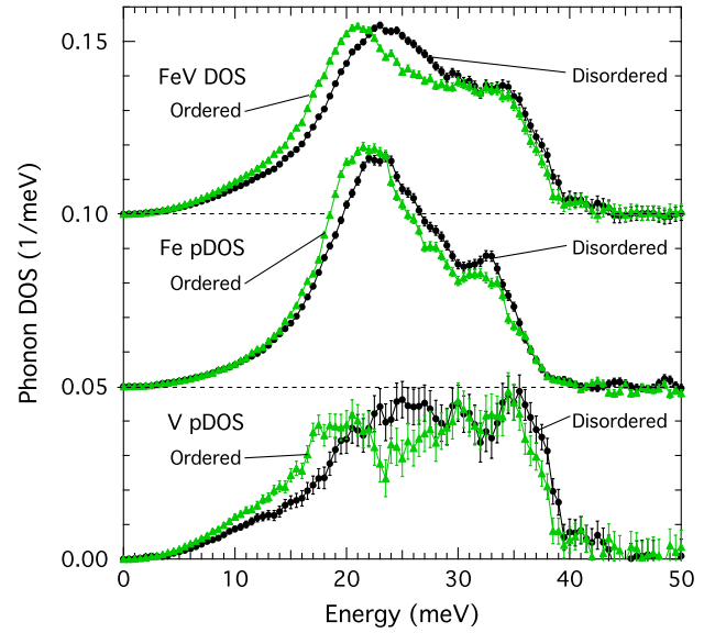
FIG. 2 (color online). Neutron-weight corrected phonon DOS curves of FeV samples (top panel), along with Fe pDOS curves (middle panel), and V pDOS curves (bottom panel). The Fe pDOS curves were determined directly by NRIXS measurements; the total FeV DOS curves and the V pDOS curves were obtained by combining INS and NRIXS spectra. Error bars are from counting statistics in the Fe pDOS, and propagation of error in the other curves.
