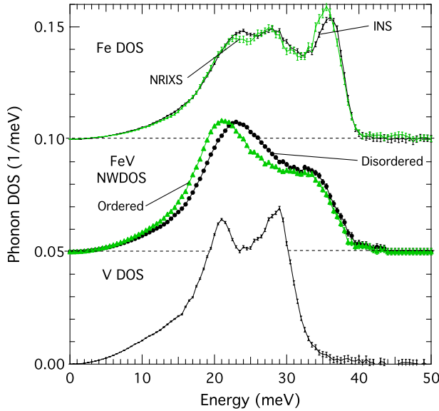
FIG. 1 (color online). Phonon DOS curves of pure Fe measured by INS and NRIXS (top panel). Neutron-weighted phonon DOS curves of FeV alloys (middle panel), and pure V (bottom panel) measured by INS. Error bars are from counting statistics.
