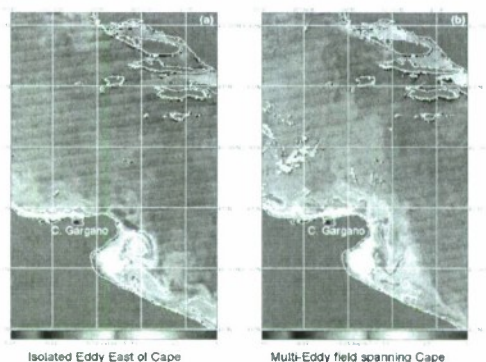
Fig. 1. Remote sensing Chlorophyll-a images from MODIS Aqua showing representative cases of (a) single anticyclonic WAC eddy downstream of Cape Gargano and (b) multiple eddy train around the Cape. This is a reproduction of Figure 2 from [1].
