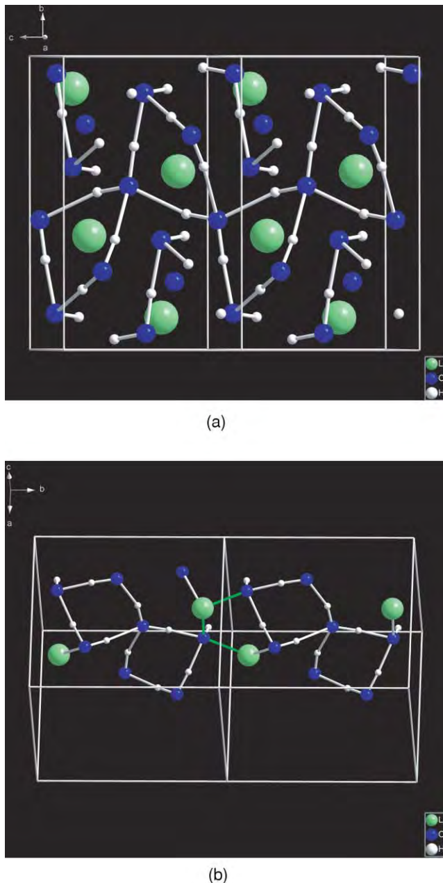
FIG. 2. (a) Representations of the structure of \text{LiOH} \cdot 2\text{H}_2\text{O} as a ball-stick model. (a) Projection along (100) . Blue: O, green: Li, white: H. White lines indicate the directions of H-bonds. The most remarkable feature of the structure is the arrangement of water molecules along (100) to a chain of four-member rings. The lack of tetrahedral coordination of all oxygen atoms but O1 violates the ice-rules and prevents macroscopic disorder of protons. (b) Atom- and bond colors as above. Green lines: Li–O distances below 2.0 \text{ \AA} , which are compatible with significant ionic interaction. The projection shows how Li resides between the \text{H}_2\text{O} tetrahedral “chains.” We note that the distances between Li and the oxygen of the hydroxide on one side and the O2 of the water molecules are shorter by only 0.04 \text{ \AA} , making Li appearing like a “network former.” However, the MD simulations indicate that \text{LiOH} \cdot 2\text{H}_2\text{O} does not behave like an itinerant ice network and does also not permit itinerant proton diffusion paths which would make this material a superb proton conductor.
