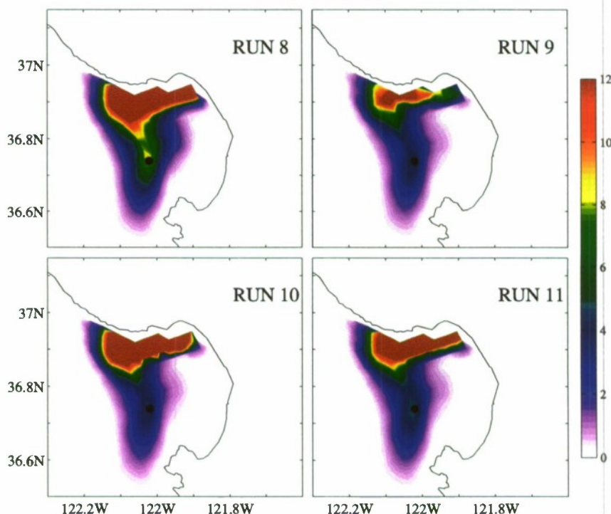
Figure 4. Vertically integrated (up to 25 m depth) concentrations maps for Runs 8–11 considered in Table 3. Integrated concentrations are at 15 August 00Z, 2003 (at 24 h of forward simulations). Values are normalized by 10^9 , units are photons m/s.
