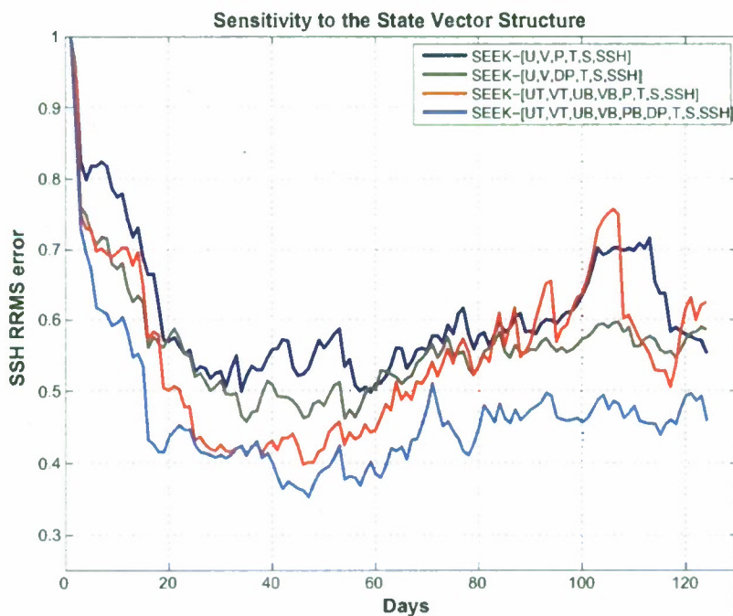
Fig. 8. Time evolution of relative RMS errors in the next day forecast SSH fields for assimilative runs with different state vector structure. The variables in the state vector for each of these runs are indicated in the figure (UT, total eastward velocity; VT, total northward velocity; DP, layer pressure thickness; P, layer interface pressure; T, layer temperature; S, layer salinity; UB, barotropic eastward velocity; VB, barotropic northward velocity; and PB, barotropic pressure). Best performance is obtained when all the variables in Table B.1 (UT, VT, UB, VB, PB, DP, T, S, SSH) are used in the estimation. Corresponding results for the other methods are similar.
