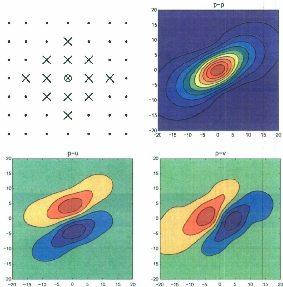
Fig. 4. The local grid domain or neighborhood \mathcal{N} of MRF coefficients in the ROIF method (x, top-left), as well as a typical datum-influence region for p field (top-right) and corresponding regions for u and v fields (bottom).
