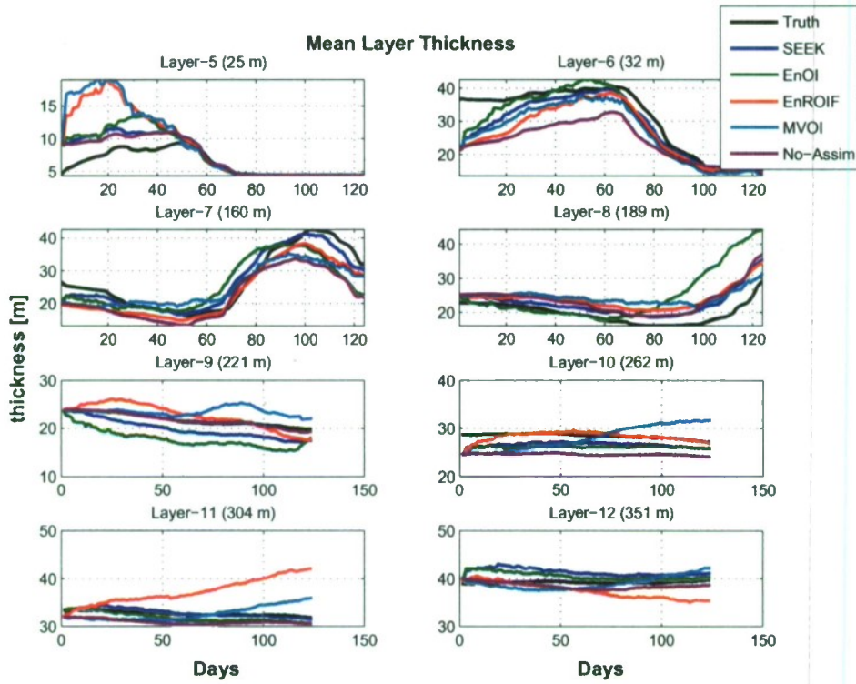
Fig. 22. Time evolution of basin averaged layer thickness in truth, the non-assimilative reference and assimilative runs in layers 5–12. The impact of assimilation is mainly seen in layer 6 where the initial basin averaged difference in layer thickness is about 20 m. The errors in this layer are reduced in the assimilative runs by 50 days compared to the non-assimilative case. The changes in the other layers are generally similar in both the assimilative and non-assimilative case (the axis scales are different for each layer). The average depth of the layer center in the Central GOM is also indicated.
