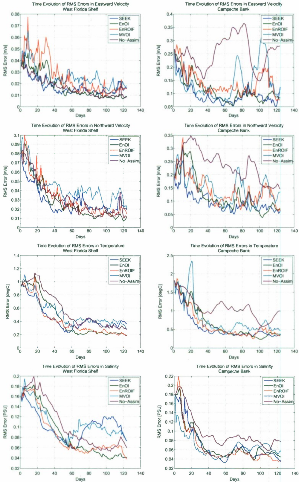
Fig. 21. Time evolution of RMS errors in U, V, T and S in two representative shallow regions. The left panels show error evolution in the West Florida Shelf region while the right panels show errors evolution in the Campeche Bank region. Both these regions are shallower than 300 m. Data in these regions are not used for assimilation. Changes to the model state in these regions are due to forcing and indirect effects of assimilation in deeper regions.
