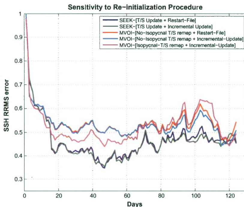
Fig. 9. Time evolution of relative RMS errors in the next day forecast SSH fields for runs using different initialization procedures. The difference in the initialization procedures are indicated in the figure. The restart file based initialization corresponds to a full insertion at one instant and subsequent integration from the restart file. Incremental updates are added over 80 time steps (6 h). T/S update in the legend corresponds to simultaneous T and S update. In all cases the best state vector structure as determined above was used.
