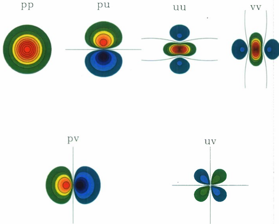
Fig. 1. Auto and cross-correlations of horizontal multivariate correlation functions for geopotential ( p ), and velocity components ( u , v ) used in the MVOI scheme. Warm (cool) colors indicate positive and negative correlations.
