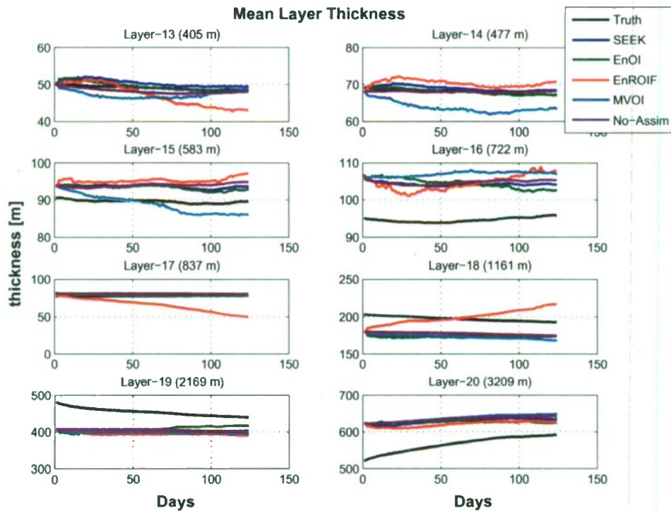
Fig. 23. Time evolution of basin averaged layer thickness in truth, the non-assimilative reference and assimilative runs in layers 13–20. The convergence to truth in these layers is generally poor (the axis scales are different for each layer) and the performance is similar to the non-assimilative case. The average depth of the layer center in the Central GOM is also indicated.
