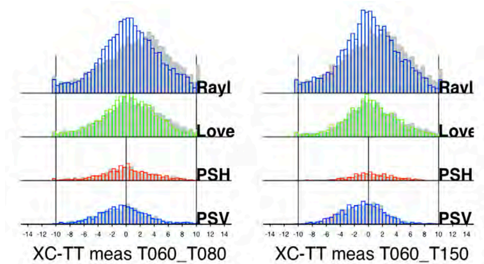
Figure 4. Comparison of travel time measurements between the initial model, gray, and the current iteration model, colors, made using cross correlation. Measurements are separated by wave type including Rayleigh (Rayl) and Love waves, and body waves on the vertical-radial components
