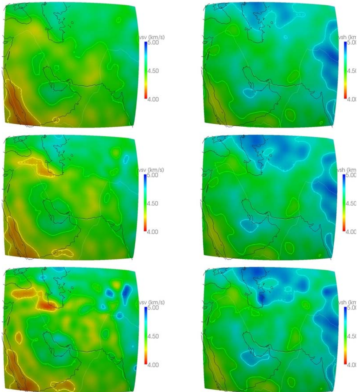
Figure 5. Comparison of the Middle East wave speed model at different iterations. The left column is Vsv and the right column is Vsh. The top row is the initial wave speed model, the second row is the 3 rd iteration and the bottom row is the 6 th iteration. Model depth is 100 km.
