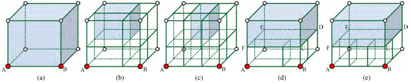
Fig. 15 An example demonstrating how to apply the templates in Figure 12(d-e) to one element with two extraordinary nodes, A and B . (a) The hexahedral element with two extraordinary nodes; (b) the result after applying the template in Figure 12(d) for node B ; and (c) the final result after applying the template in Figure 12(d) for node A . Similarly, (d-e) shows the two results after applying the template in Figure 12(e) first for node B and then for node A .
