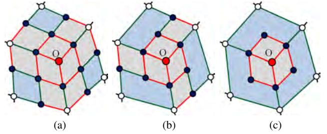
Fig. 10 1-ring and 2-ring neighborhoods around an extraordinary node O in the T-mesh after applying the four template sets in Table 1. (a) set 1; (b) sets 2 and 3; and (c) set 4.
