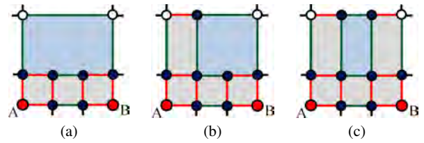
Fig. 7 Three possible results for element type 2 (sets 2 and 3) after applying the template in Figure 5(b) by choosing different orientations.
