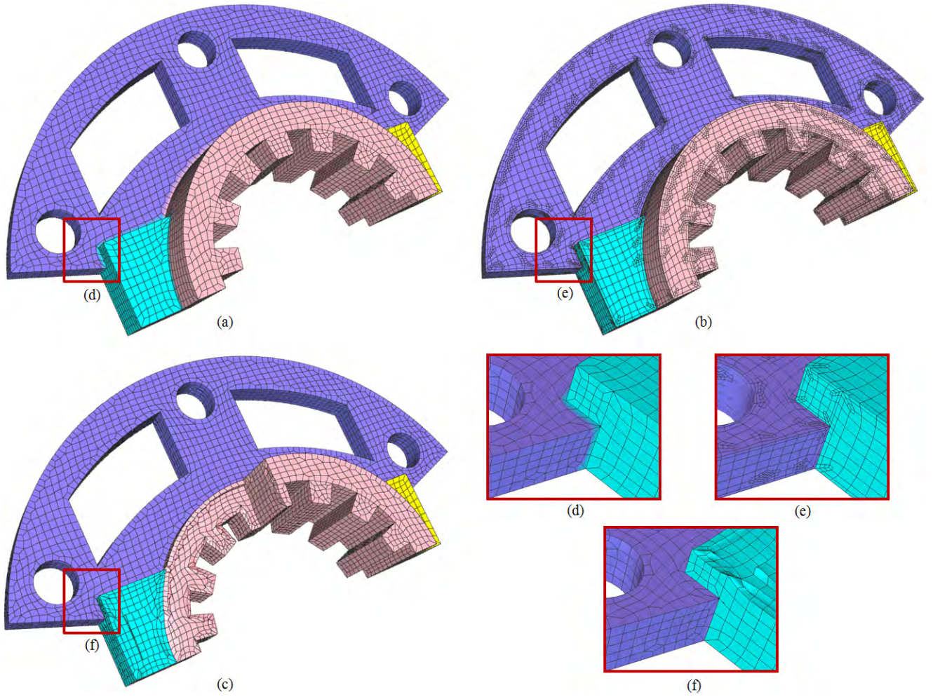
Fig. 1 The gear assembly. (a) The input unstructured hexahedral mesh; (b) the constructed solid T-spline and T-mesh; and (c) the extracted solid Bézier elements with some elements removed to show the interior mesh. (d-f) show details.
