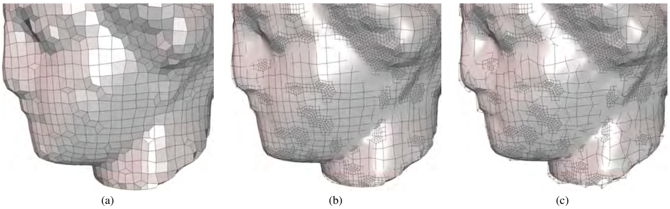
Fig. 18 Surface fitting for a solid T-spline model. (a) The input hexahedral mesh; (b) the constructed solid T-spline and T-mesh before surface fitting; and (c) the constructed solid T-spline and T-mesh after surface fitting.
