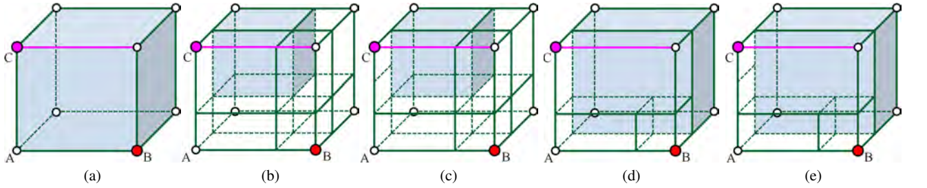
Fig. 16 An example demonstrating how to apply the templates in Figure 12(c-e) to one element with one extraordinary node B and one partial extraordinary node C . (a) The hexahedral element in which the magenta edge has one reflection edge about node C ; (b) the result after applying the template in Figure 12(d) for node B ; and (c) the final result after applying the template in Figure 12(c) for node C . Similarly, (d-e) show the two results after applying the template in Figure 12(e) first for node B and then the template in Figure 12(c) for node C .
