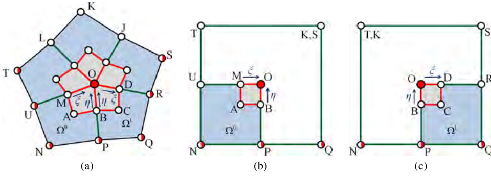
Fig. 9 A local region around one valence-5 extraordinary node O . (b) and (c) show the nodes around the extraordinary node with non-zero basis function values and their parametric position for domains \Omega^0 and \Omega^1 .
