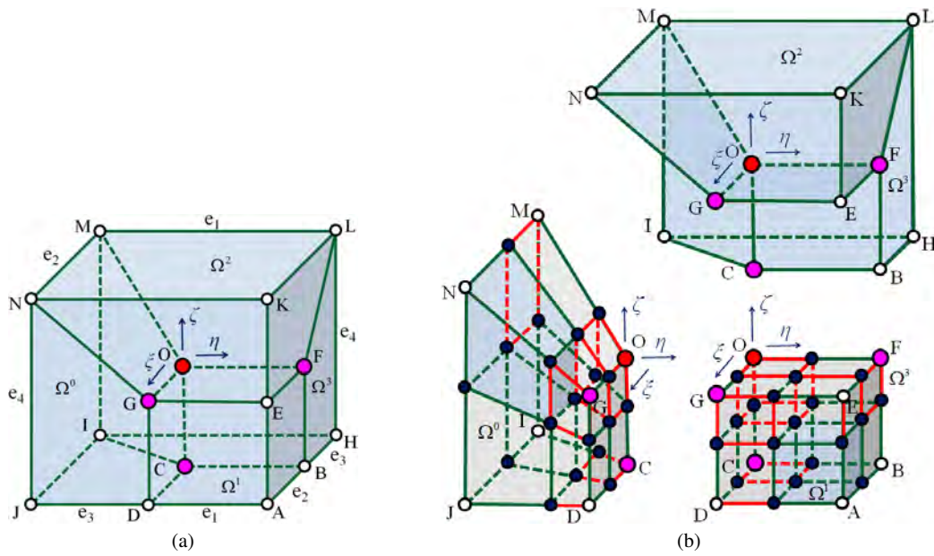
Fig. 14 One local region with an extraordinary node O . (a) shows the input hexahedral mesh and (b) is the exploded view of the T-mesh after applying the template in Figure 12(d). Node O is the parametric origin.
