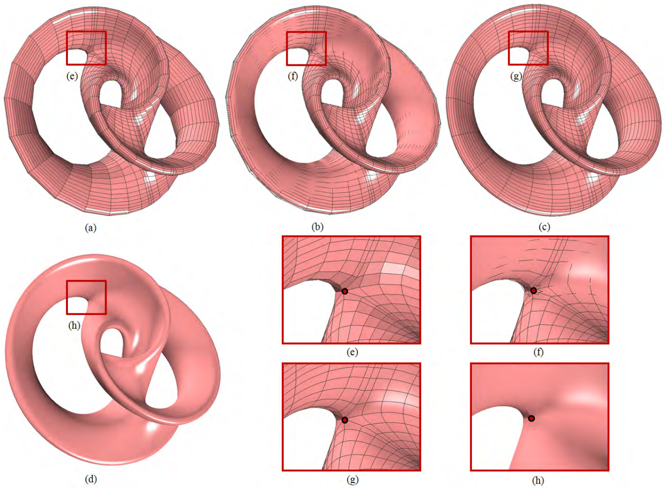
Fig. 19 One genus-3 model. (a) The input unstructured quadrilateral mesh; (b) the constructed T-spline surface and T-mesh; (c) the extracted Bézier elements; and (d) the T-spline surface. (e) to (h) show details.
