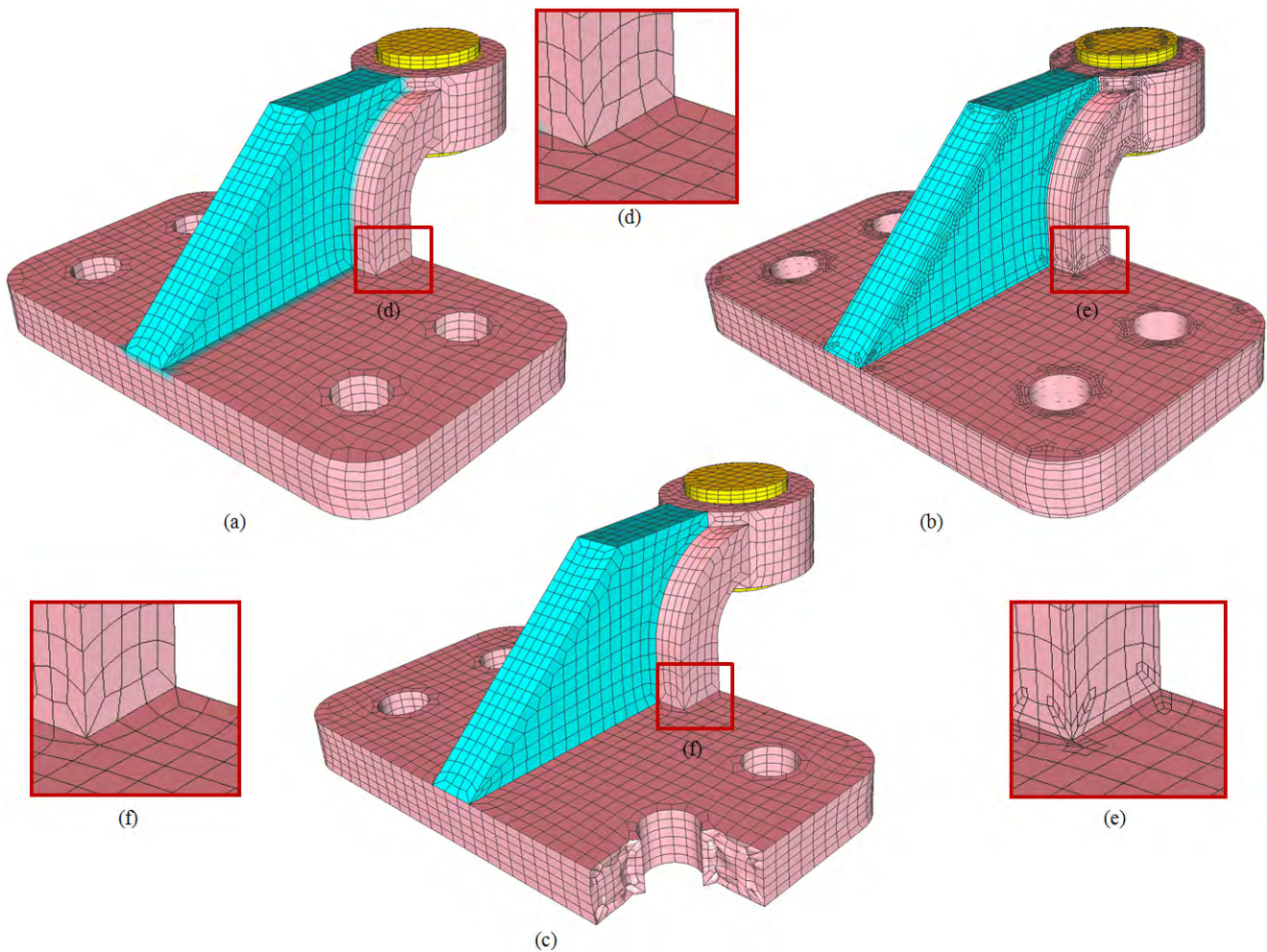
Fig. 25 The bearing assembly. (a) The input unstructured hexahedral mesh; (b) the constructed solid T-spline and T-mesh; and (c) the extracted solid Bézier elements with some elements removed to show the interior mesh. (d) to (f) show details.
