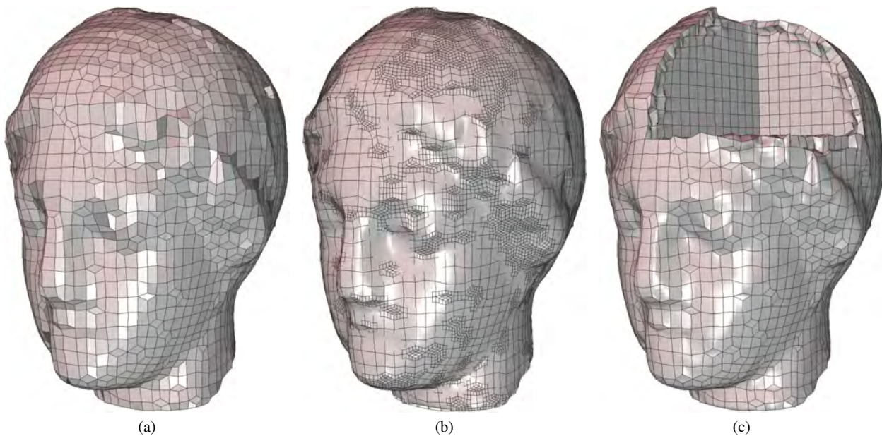
Fig. 24 One statue model. (a) The input unstructured hexahedral mesh; (b) the constructed solid T-spline and T-mesh; and (c) the extracted solid Bézier elements with some elements removed to show the interior mesh.
