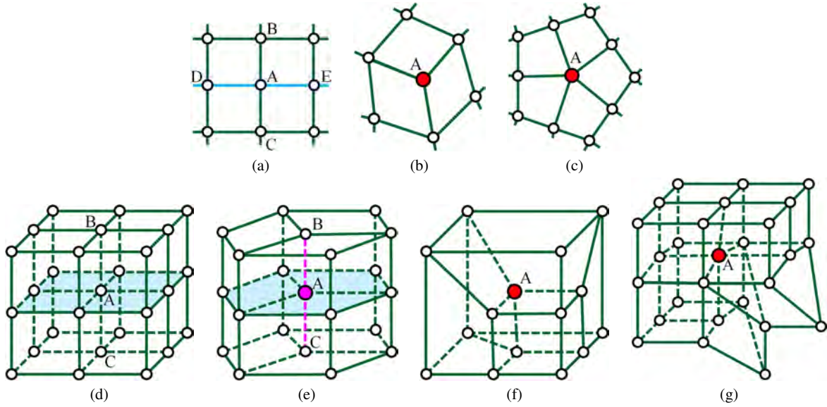
Fig. 4 Regular node, partial extraordinary node and extraordinary node in 2D and 3D. Node A rendered in white is a regular node (a, d), the magenta node is a partial extraordinary node (e), and red nodes are extraordinary nodes (b, c, f and g).
