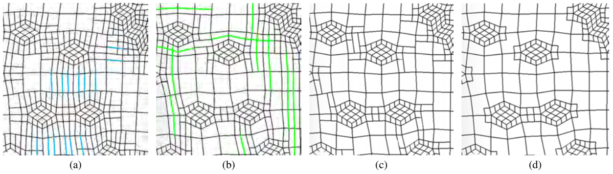
Fig. 11 A comparison of using template sets 1-4. (a) The rational T-mesh after applying set 1; (b) the standard T-mesh after applying set 2 and standardization; (c) the rational T-mesh after applying set 3; and (d) the rational T-mesh after applying set 4.
