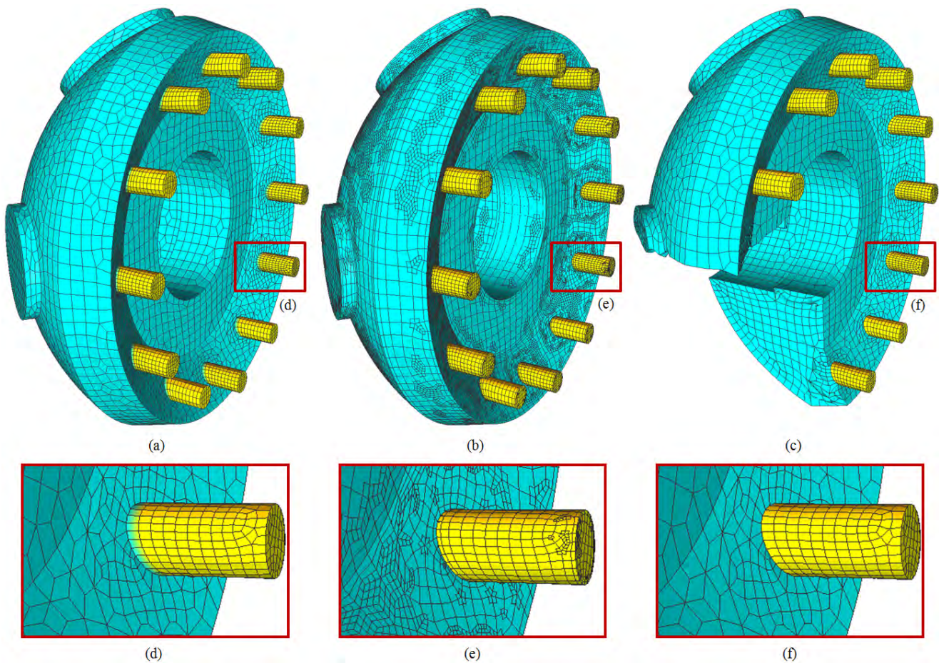
Fig. 26 The eddy plate assembly. (a) The input unstructured hexahedral mesh; (b) the constructed solid T-spline and T-mesh; and (c) the extracted solid Bézier elements with some elements removed to show the interior mesh. (d) to (f) show details.
