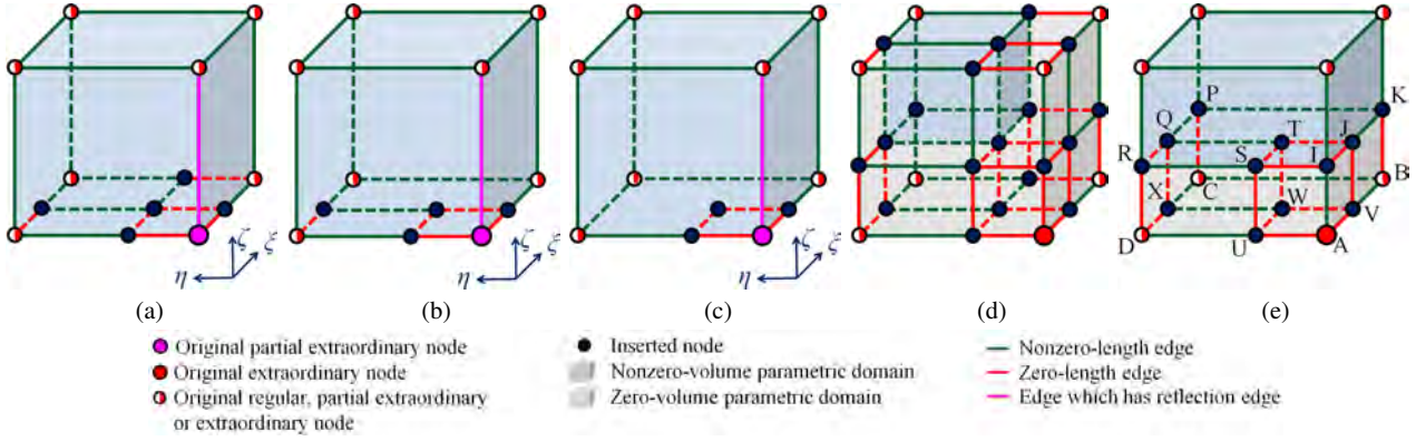
Fig. 12 The general templates for partial extraordinary nodes (a-c) and extraordinary nodes (d-e) of hexahedral meshes. (a-c) are generalized from templates in Figure 5(a-c), respectively; (d) is extended from the template in Figure 5(a); and (e) is a simplified version of (d).
