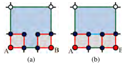
Fig. 8 The template derivation process for element type 2 (set 4) from the template in Figure 5(c). (a) The result after applying the template to the extraordinary nodes A and B ; and (b) the final result after adding the blue edge according to a T-spline rule.
