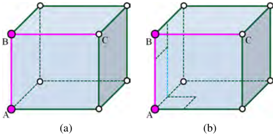
Fig. 13 One element with two partial extraordinary nodes, A and B . (a) The input hexahedral element in which edge AB has one reflection edge about A and edge BC has one reflection edge about B ; and (b) the result after applying the template in Figure 12(c) to nodes A and B .
