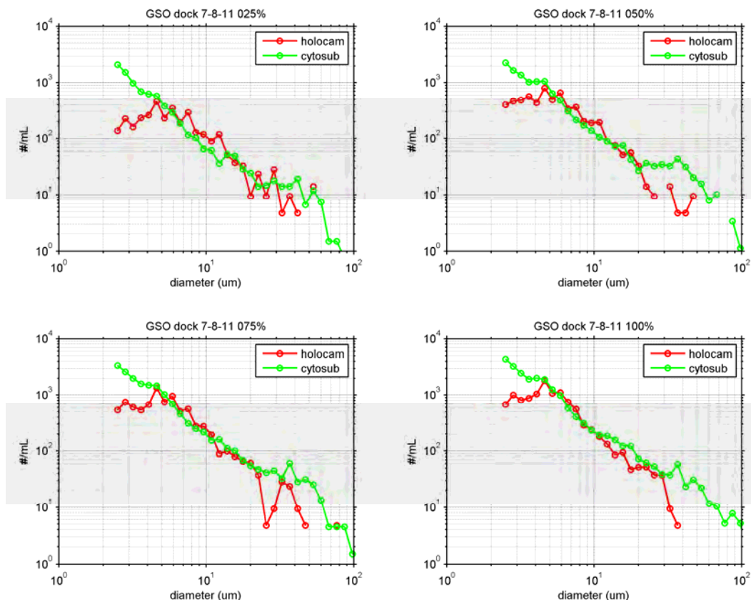
Figure 4. Particle size distribution (PSD) comparisons between the bench-top HOLOCAM and a Cytosub flow cytometer using four dilutions of a natural water sample from Narragansett Bay, RI. The bench-top HOLOCAM is optimized for particle sizes > ~ 4 to 5 \mu\text{m} and the Cytosub for particles > ~ 2 \mu\text{m} . The PSDs compare very well within the working measurement ranges of these devices.
