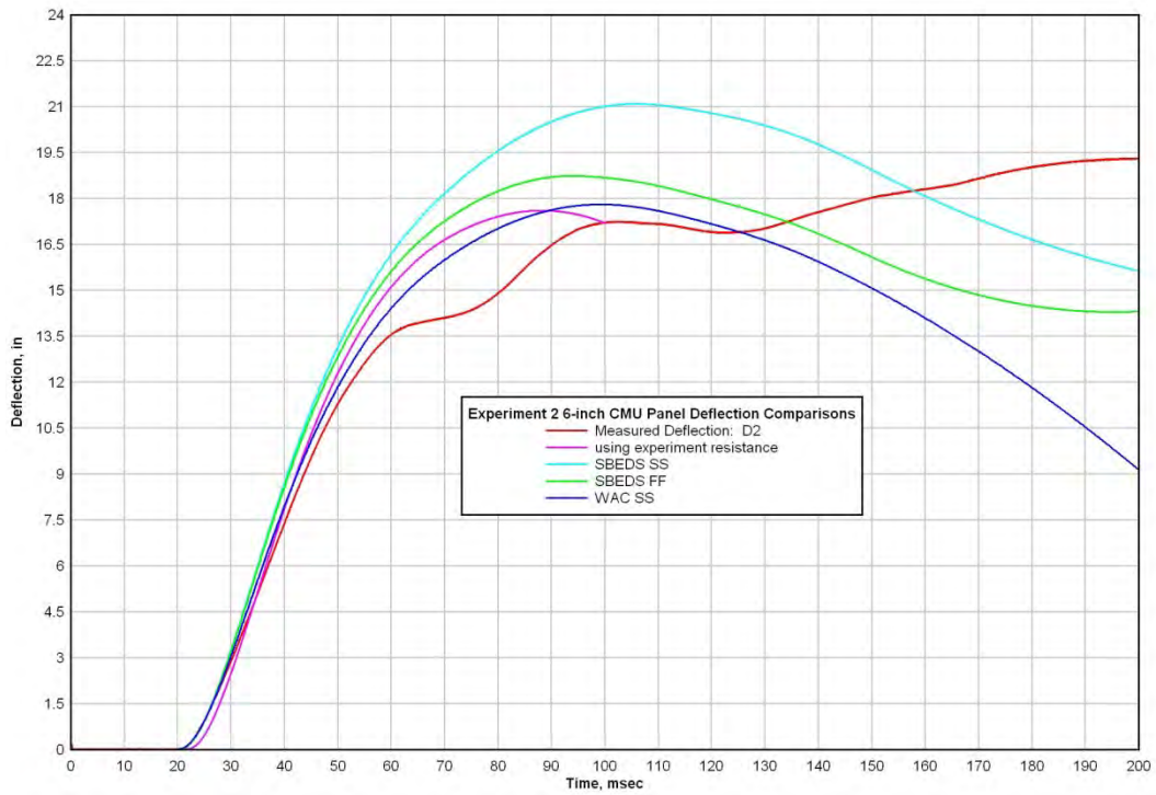
Figure 68. Experiment 2 6-inch CMU Panel Analytical and Experimental Dynamic Response Comparisons
