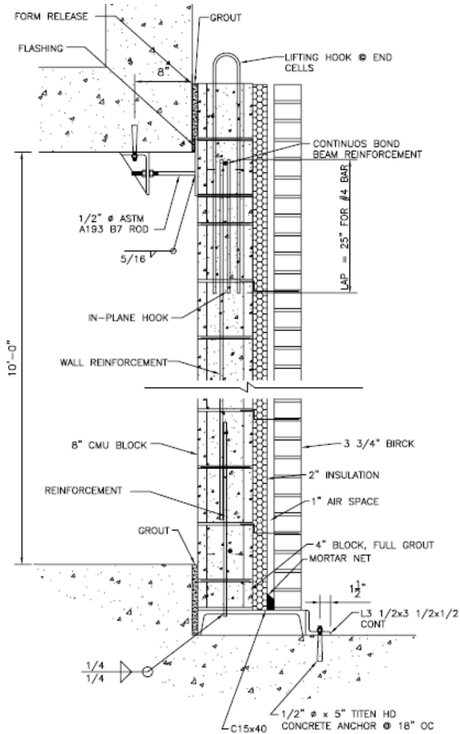
Figure 6. Cavity Wall Panel Design
