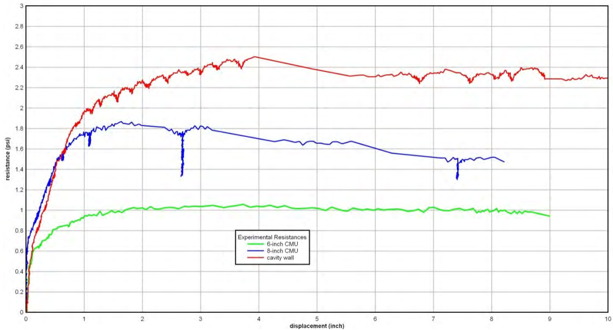
Figure 62. Experimental Static Resistance Results
