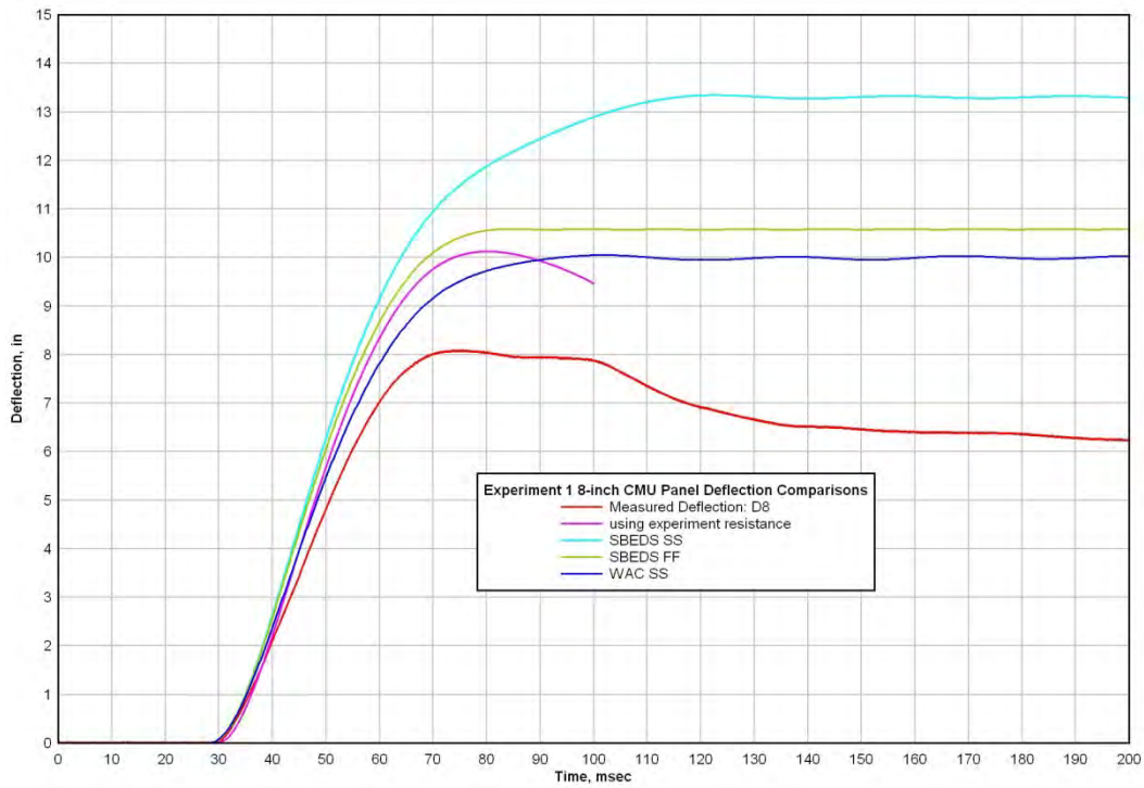
Figure 66. Experiment 1 8-inch CMU Panel Analytical and Experimental Dynamic Response Comparisons
