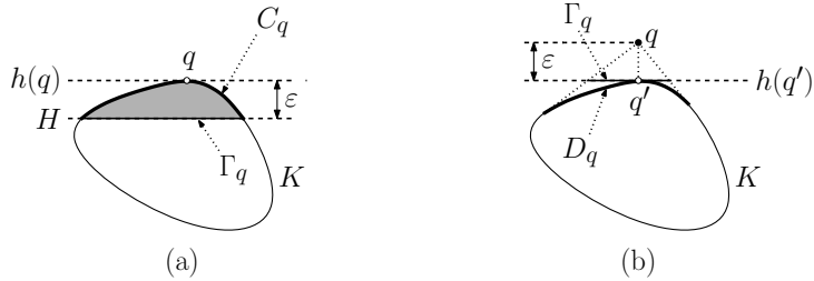
Figure 2: Caps and dual caps.
