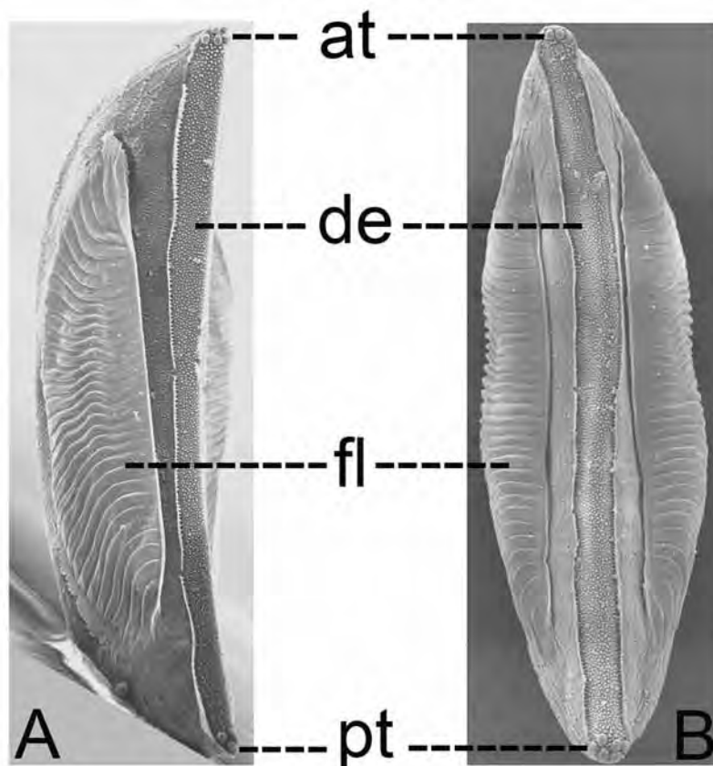
FIGURE 2. Lateral (A) and ventral (B) views of An. sineroides egg, showing general morphological parts, 200x. Abbreviations used include at = anterior tubercles, de = deck, fl = float (with ribs), pt = posterior tubercles.
