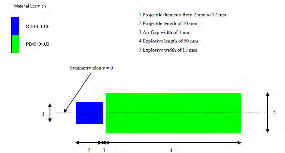
Figure 12: Disposal designed in AUTODYN® to simulate the Moulard experiment.
