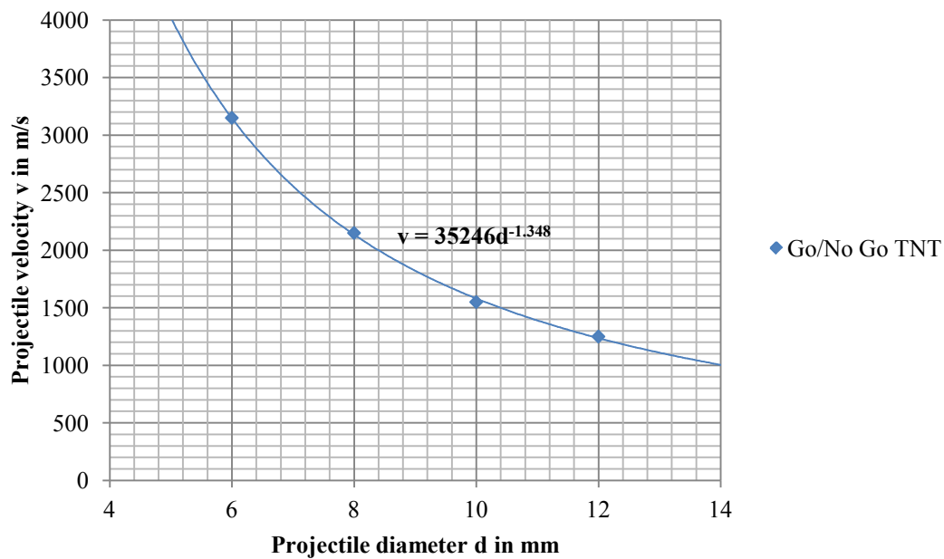
Figure 39: "Go/No Go" velocities as a function of the projectile diameter. Simulation results obtained for a steel projectile impacting a bare block of explosive TNT by a zoning of 2 cells/mm.
