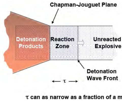
Figure 8 [021]: Evolution of the detonation wave front in the explosive.
