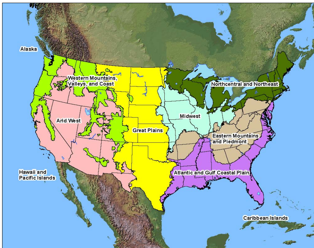
Figure 1. U.S. Army Corp of Engineers Wetland Delineation Regions.
