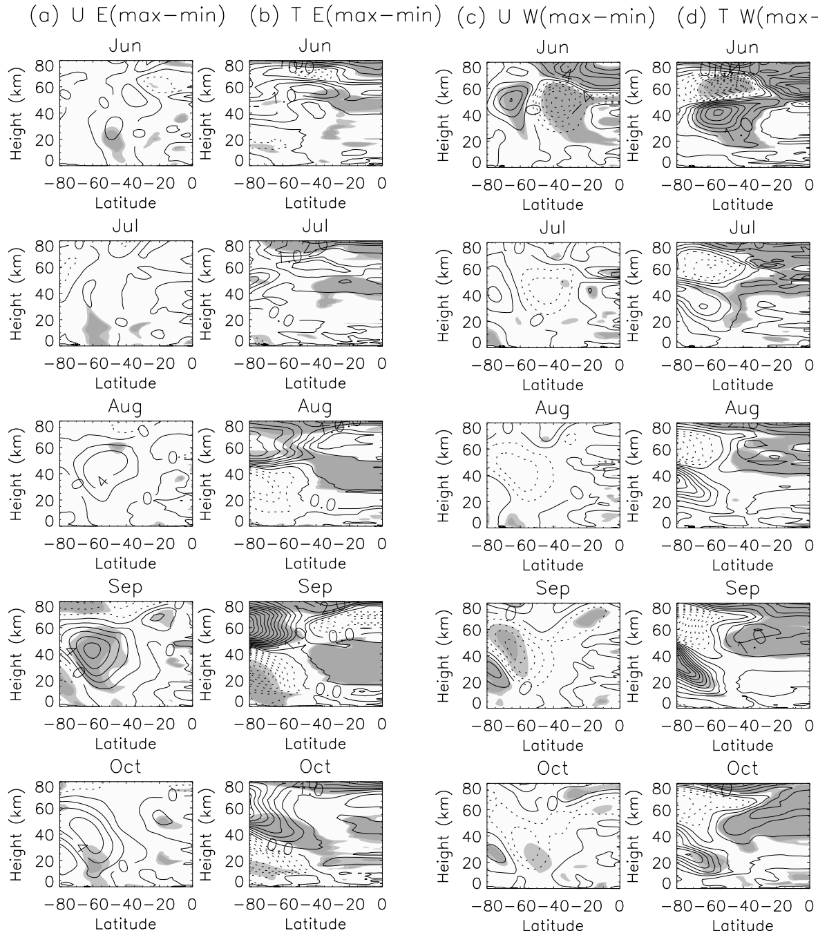
Figure 10. June through October temperature and zonal-mean zonal wind differences between solar maximum and minimum for the (a and b) QBO east (maxE minus minE) and (c and d) QBO west (maxW minus minW) experiments; shading as in Figure 4.
