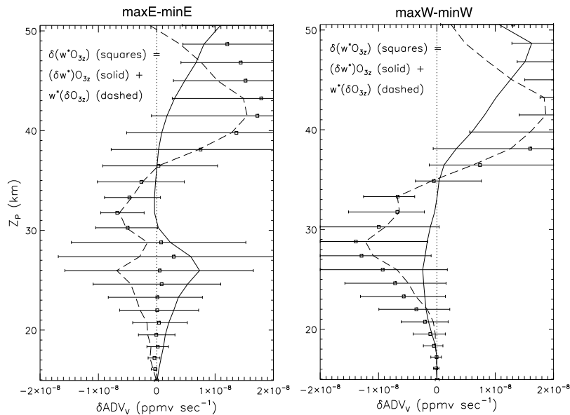
Figure 9. Change in vertical advection of ozone, -w^*\partial O_3/\partial z , between solar minimum and solar maximum (squares) for (left) QBO-east and (right) QBO-west, together with the contribution from changes in vertical velocity (solid lines) and changes in the vertical gradient of ozone (dashed lines). See section 5.2 for details.
