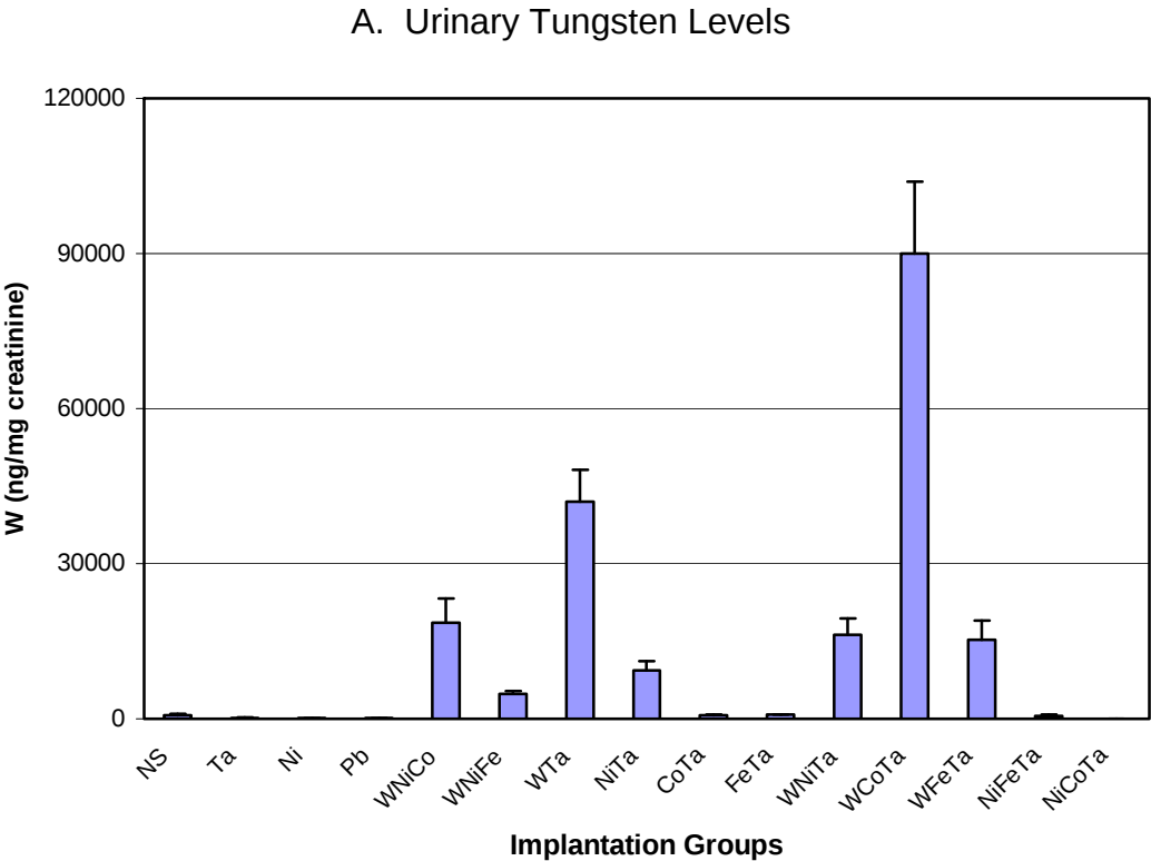
Figure 12: Urinary Metal Levels in 1-Month Implantation Groups
