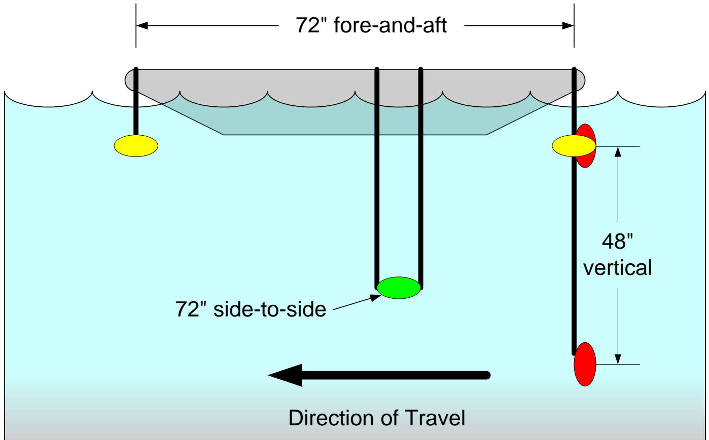
Figure 7. Configuration of electrode sensor array with color-coded electrode pairs.
