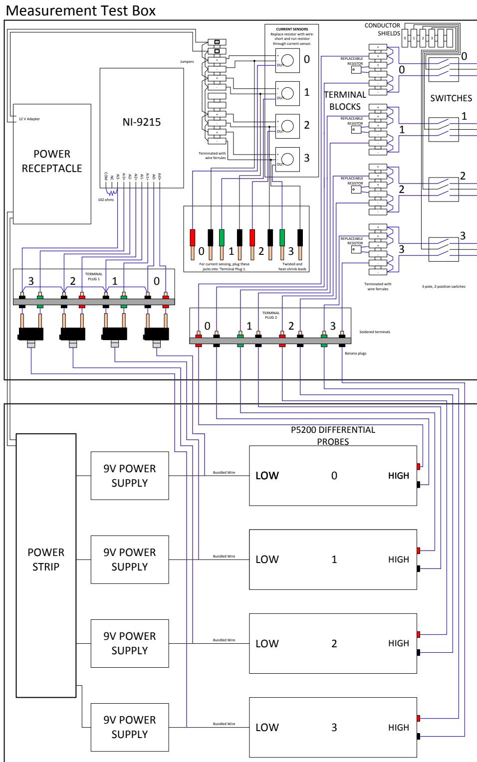
Figure A-1. Measurement test box schematic diagram.
