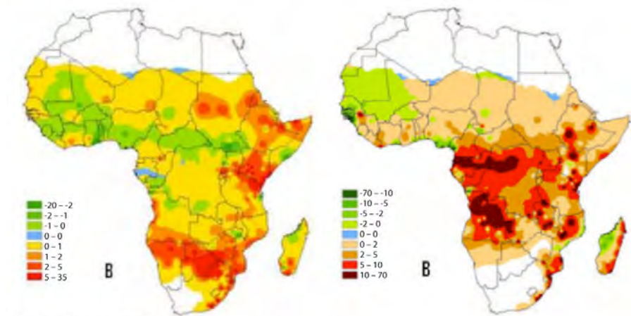
Figure 3-10. Change in distribution of the two most prevalent malaria vectors ( Anopheles mosquitoes) for a rise of 2°C Africa wide temperature, 10% increase of summer rainfall, and 10% decrease in winter rainfall
