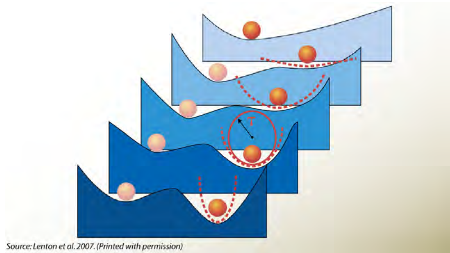
Figure B-2. Concept view of a tipping point or threshold crossing event leading to an abrupt change in climate state and future stability
