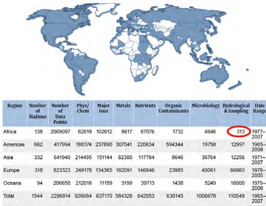
Figure1-4. Comparison of hydrologic observation sites for UNEP GEMS program
