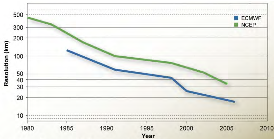
Figure 1-2. Trends in short-term weather (0-14 Days) numerical weather prediction resolution
