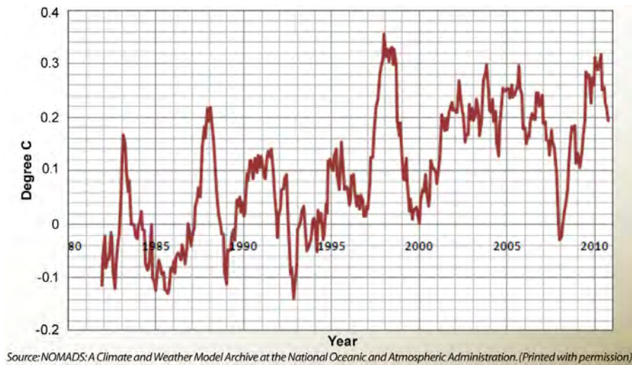
Figure 2-3. Global Optimum Interpolation (OI) SST anomalies (OI.v2) (November 1981 to September 2010) 27
