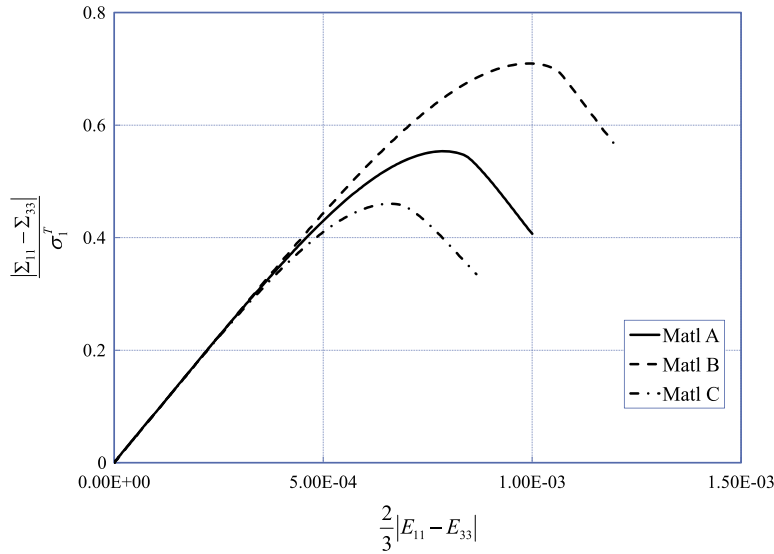
Fig. 10. Typical von Mises effective stress versus von Mises effective strain curves corresponding to FE calculations at T_E = 1.5 and with the major stress in the \mathbf{e}_3 direction. For all materials the yield stress in tension and compression are equal ( k = 0 ) with material type A being isotropic ( \sigma_1^{T,C} = \sigma_3^{T,C} ), material type B having a through-thickness yield strength greater than the in-plane yield strength ( \sigma_1^{T,C} < \sigma_3^{T,C} ) and material type C having a through-thickness yield strength lower than the in-plane yield strength ( \sigma_1^{T,C} > \sigma_3^{T,C} ).
