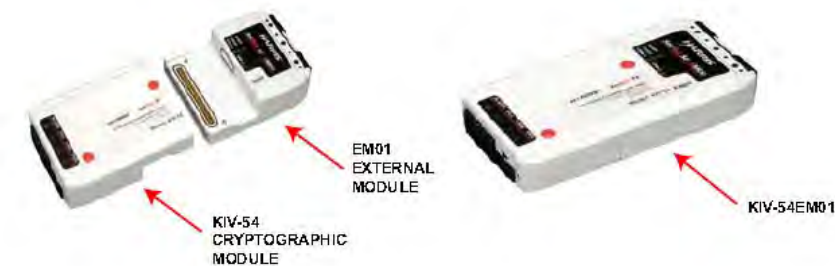
Figure 3. SecNet54 Cryptographic Module and Ethernet Module. From [17].
