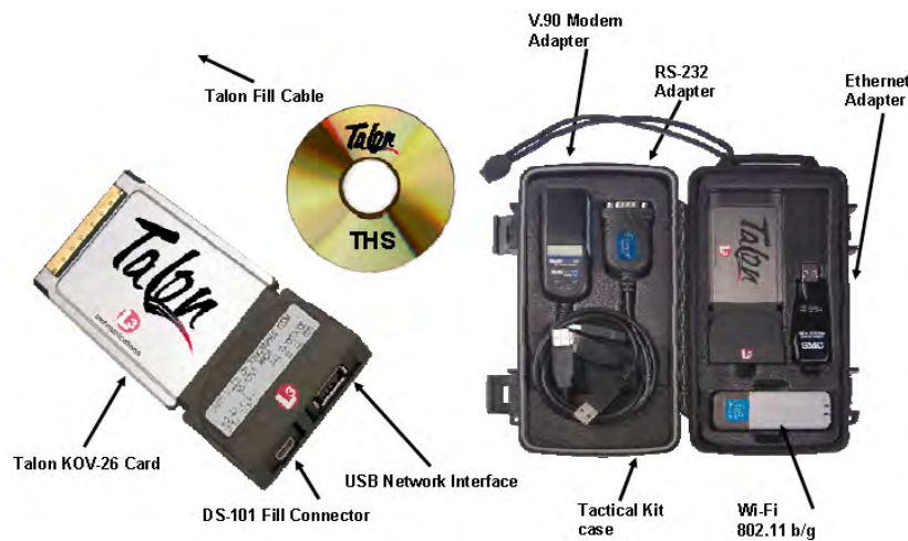
Figure 1. The Talon and Its Tactical Kit Accessories. From [11].
