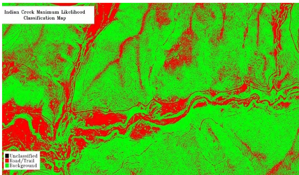
Figure 65. Maximum Likelihood Classification result, no probability threshold, applied to Indian Creek survey area. The red areas are classified as most likely to be road/trail. The green areas are classified as most likely to be other than road/trail.
