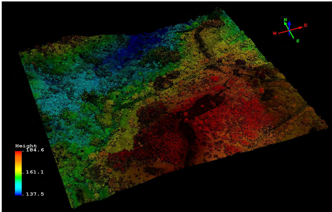
Figure 36. Kahuku point cloud, all returns. Colors show relative elevation values in meters.
