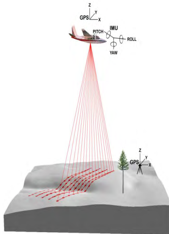
Figure 2. Rangefinding scanning and aircraft orientation (From McGaughey, Andersen, & Reutebuch, 2006)
