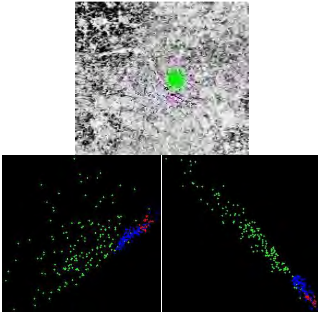
Figure 67. Regions (top) drawn over MNF band 1 image, red points identified as most likely trail, blue points as possibly trail, and green as not trail. N-D visualizer scatter plot (lower left) utilizing MNF bands 1 through 4, and scatter plot (lower right) utilizing MNF band 1 and band 2.
