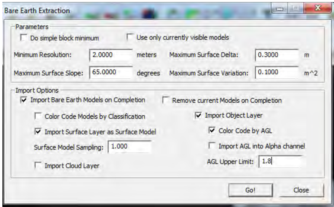
Figure 38. Bare earth extraction import menu.
