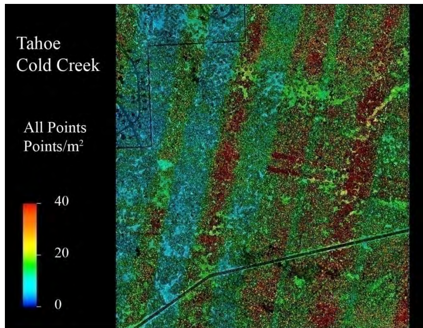
Figure 50. Lake Tahoe, Cold Creek survey area Number of Points for all points. Flight line overlap effects are clearly evident as strips of higher density points transiting the image.
