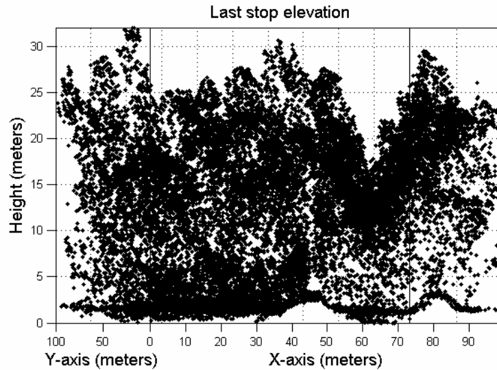
Figure 26. Point cloud cross section from study area where small empty space above trail surface is visible (between 40 m and 50 m on X-axis) (After Heezin Lee et al., 2005).
