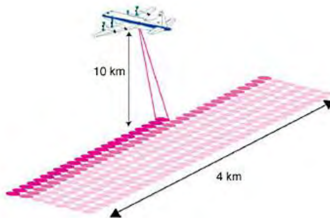
Figure 17. Example of swath implemented by LVIS (From National Aeronautics and Space Administration [NASA], 2011b)
