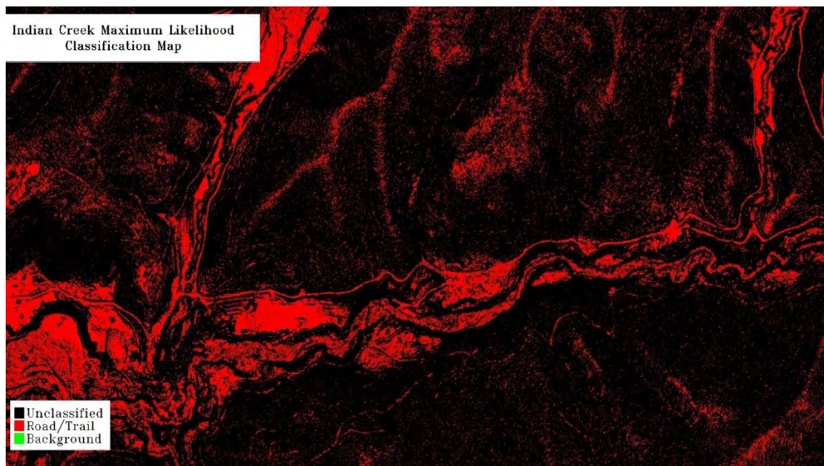
Figure 64. Maximum Likelihood Classification result, probability threshold of 10%, applied to Indian Creek survey area. The red areas are classified as most likely to be trail. Vast areas of the survey area are unclassified at this threshold.
