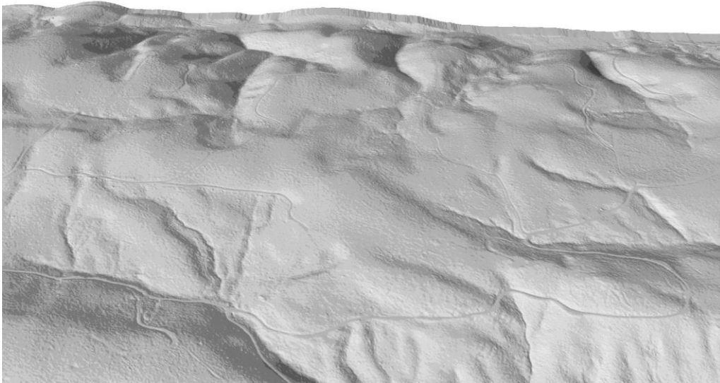
Figure 6. DEM formed from LiDAR survey under multistoried forest canopy (From Reutebuch, Andersen, & Carson, 2003)
