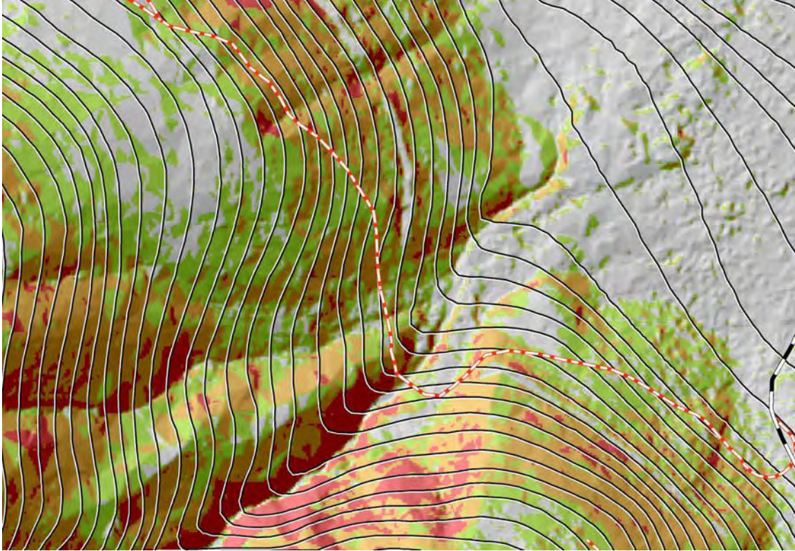
Figure 13. Contour lines overlayed on LiDAR-derived DEM with slope class coloring revealing the greater detail available than from working with Topographic map alone (After Krogstad & Schiess, 2004)
