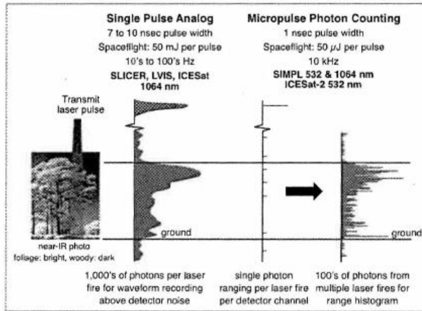
Figure 23. Comparison between conventional single pulse full waveform systems and micropulse photon counting systems measurement approaches of forest canopy structure (From Harding et al., 2011)
