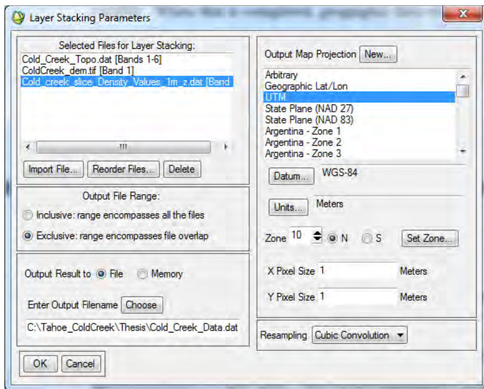
Figure 58. Layer Stacking Parameters input menu. Files are selected for stacking in order of precedence and output in re-sampled, 1 m 2 pixels.
