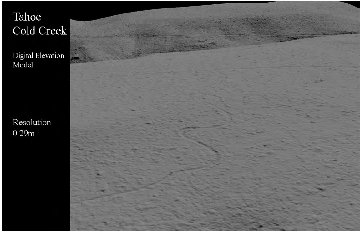
Figure 47. Birds-eye view of DEM in Lake Tahoe, Cold Creek with trail clearly visible winding across the landscape corresponding to linear gap in point cloud absent of points from Figure 46.
