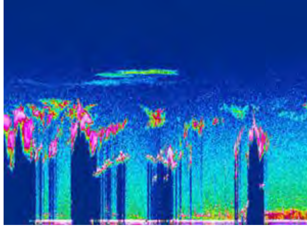
Figure 3. CALIPSO LiDAR collection, June 2006 from sea level to 30km (From National Aeronautics and Space Administration [NASA], 2011)
