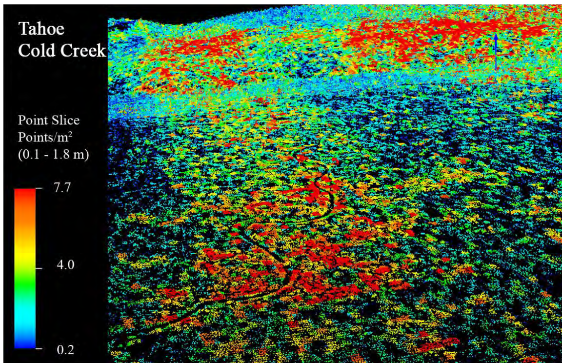
Figure 46. Birds-eye view of 3D point cloud in Lake Tahoe, Cold Creek from 0.1m to 1.8m. Linear gap in point cloud absent of points is clearly visible winding across the landscape, corresponding to identifiable trail on the DEM in Figure 47
