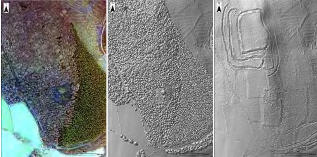
Figure 14. Prehistoric, fortified enclosure known as Welshbury Hill in the Forest of Dean, Gloucestershire, UK. Left image from digital imagery, center image is a LiDAR DTM, and right image is an extracted DEM (After Devereux et al., 2005)
