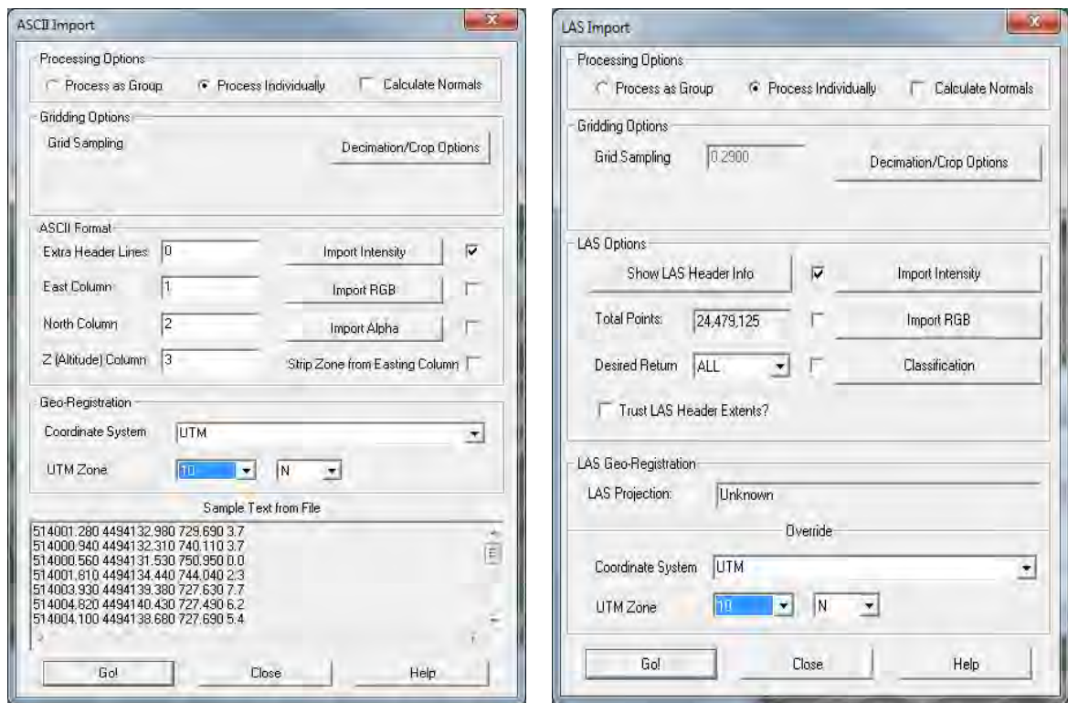
Figure 31. ASCII dataset import menu on the left and LAS dataset import menu on the right. For ASCII, data is arranged as text in file by column as East, North, Z, and Intensity. For LAS, data can be imported with intensity or according to classification.
