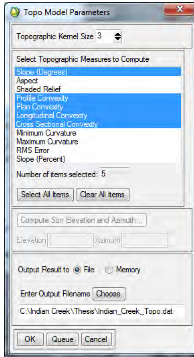
Figure 52. Topographic model parameters, selection of measures to compute, kernel Size and output to file.
