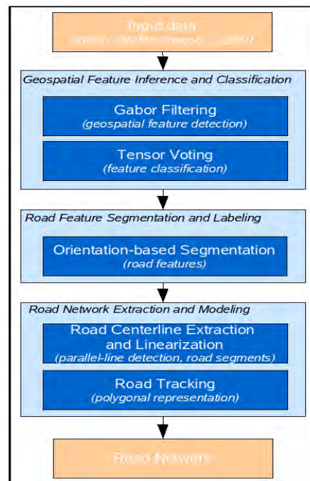
Figure 25. Vision-based system overview for automatic detection and extraction of road networks (From Poullis, 2008).
