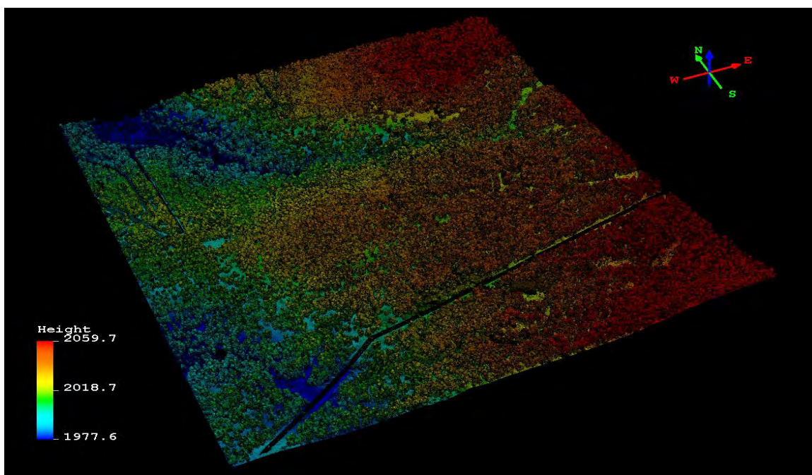
Figure 34. Lake Tahoe, Cold Creek point cloud, all returns. Colors show relative elevation values in meters.
