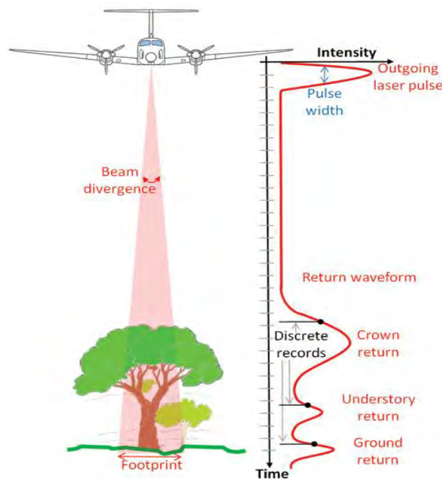
Figure 4. Illustration of LiDAR waveform and discrete recording characteristics (From Diaz, 2011)
