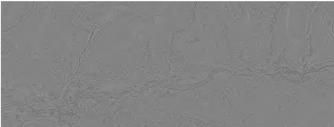
Figure 54. Indian Creek topographic profile convexity band.
