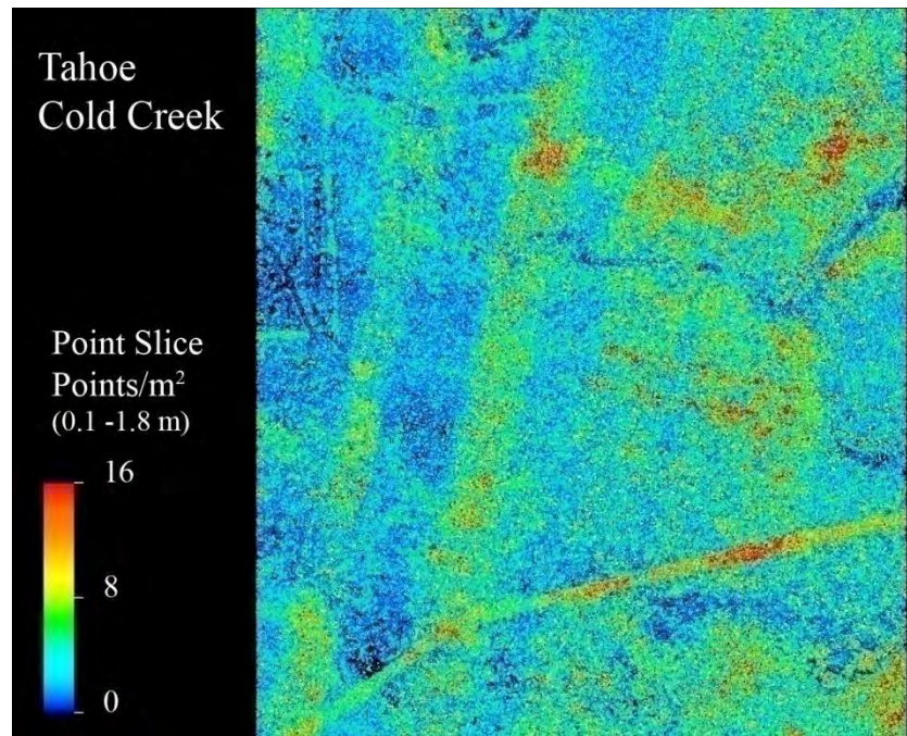
Figure 51. Lake Tahoe, Cold Creek survey area Number of Points for 0.1 m to 1.8 m AGL point cloud slice. Flight line overlap effects are clearly evident
