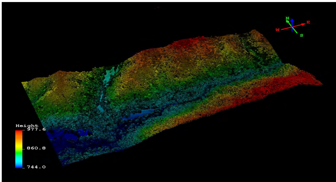
Figure 32. Indian Creek point cloud, all returns. Colors show relative elevation values in meters.
