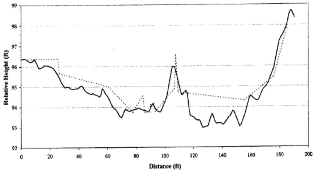
Figure 20. Example comparing river crossing profile of ground survey (dashed line) with LiDAR data results (solid line) (From Coutermarsh, 2003)
