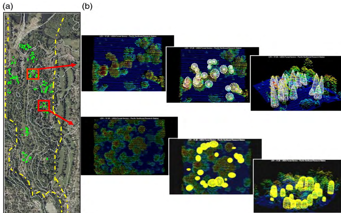
Figure 7. Display shows (a) Location of individual trees plotted over aerial photography and (b) LiDAR point clouds of individual trees selected out for study based on intensity values. Conifers are on top displayed in white, broadleaved species below displayed in yellow (From Kim et al., 2009)
