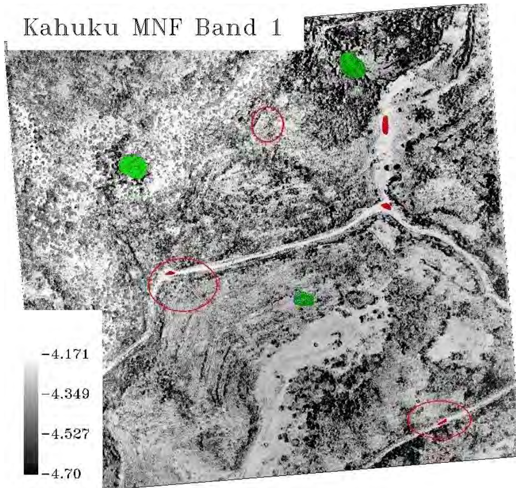
Figure 70. Kahuku survey area, Regions of Interest over MNF band 1, identifying roads/trails (red selections) and nonroads/trails (green selections). Differing shades of red and green are the result of further n-D visualizer analysis.
