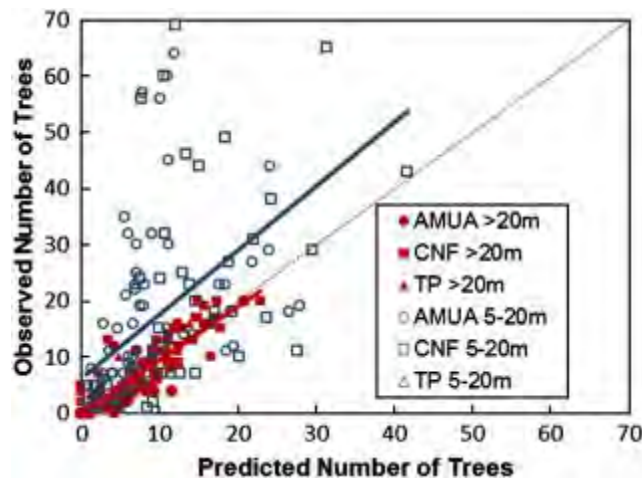
Figure 11. Comparison of predicted tree density to field measured tree density for all polts measured in the study for two height classes. The red icons are for trees greater than 20 m tall and the blue icons are for trees between 5m and 20 m tall. Locations are the Ahtanum Multiple Use Area (AMUA), Colville National Forest (CNF), and Training Plots (TP) (From Richardson & Moskal, 2011).
