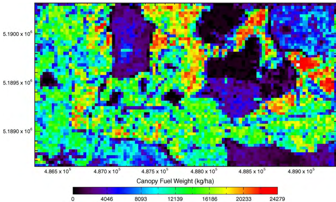
Figure 10. LiDAR derived forest canopy fuel weight map (30 m resolution) (From Andersen, McGaughey, & Reutebuch, 2005)
