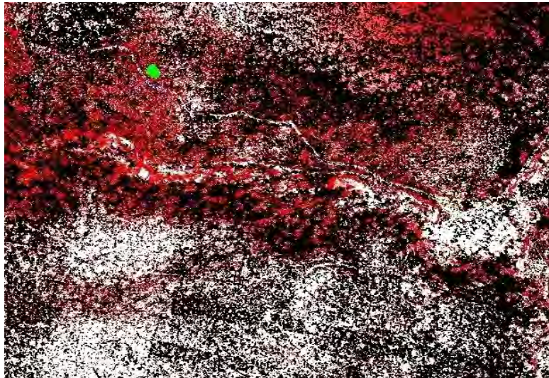
Figure 69. Subset of Lake Tahoe, Cold Creek survey area surrounding region of interest selected areas (upper left of figure that includes the green shaded region of nontrail points). Classified such that the whiter the area, the more likely it is a trail.
