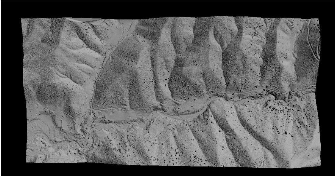
Figure 40. Digital Elevation Model from Indian Creek watershed survey area revealing surface features beneath vegetation.
