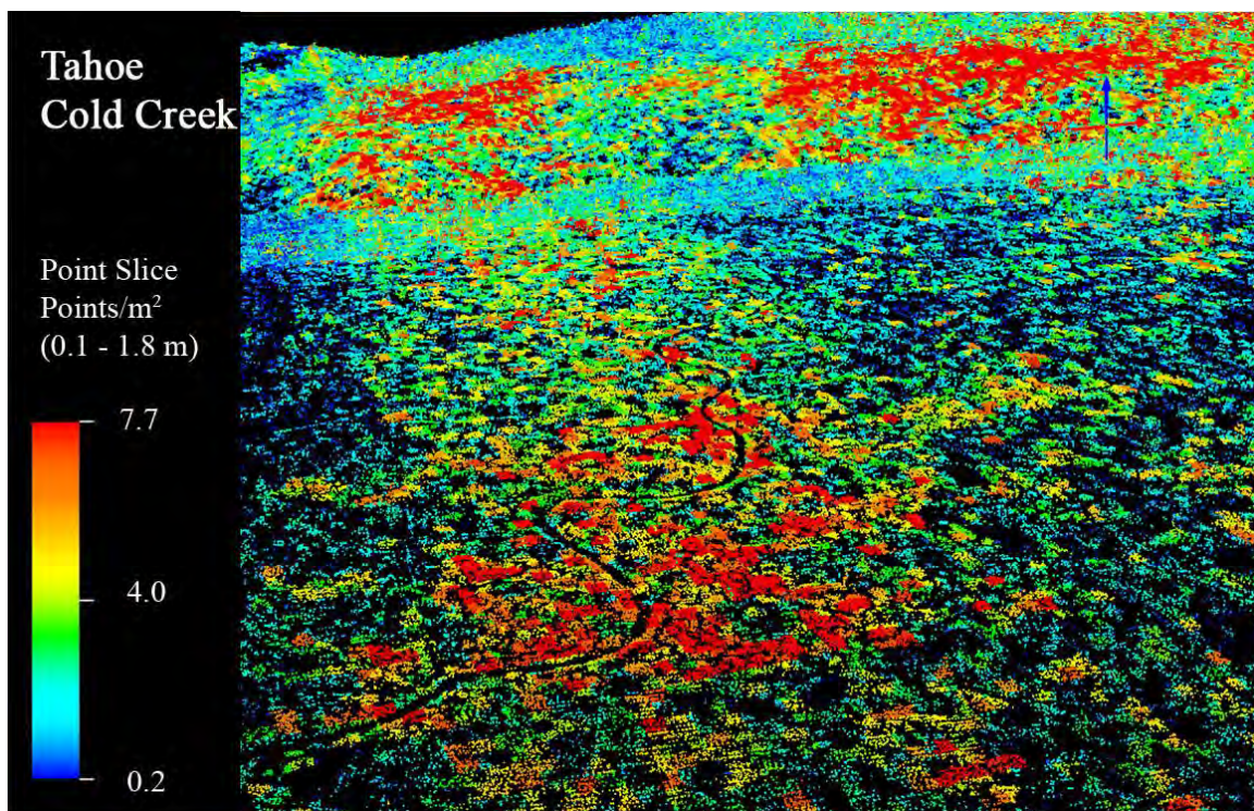
Figure 74. Birds-eye view of 3D point cloud in Lake Tahoe, Cold Creek from 0.1m to 1.8m. Linear gap in point cloud absent of points is clearly visible winding across the landscape, corresponding to identifiable trail on the DEM
