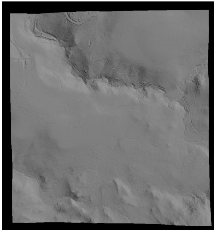
Figure 42. Digital Elevation Model from Cold Creek survey area in Lake Tahoe Basin revealing surface features beneath vegetation
