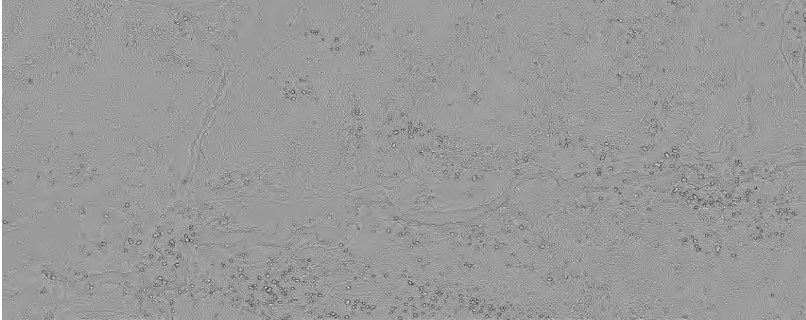
Figure 56. Indian Creek topographic longitudinal convexity band.
