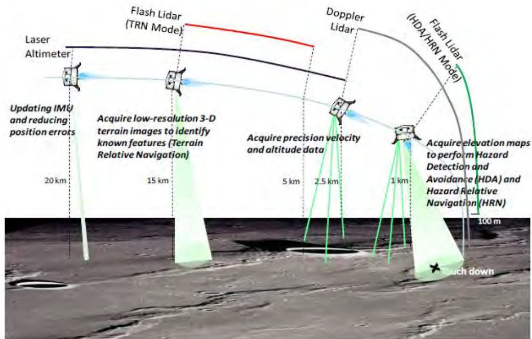
Figure 21. Example of how Laser landing sensors could be utilized in spacecraft landing scenarios (From Amzajerian et al., 2011)
