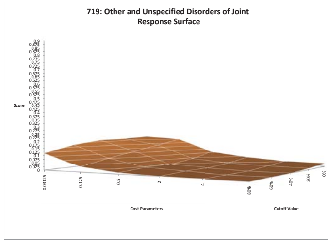
Figure B.12: The F -score response surface of 719 created by the tuning of the cost parameter and the confidence cutoff for term frequency-inverse document frequency weighting
