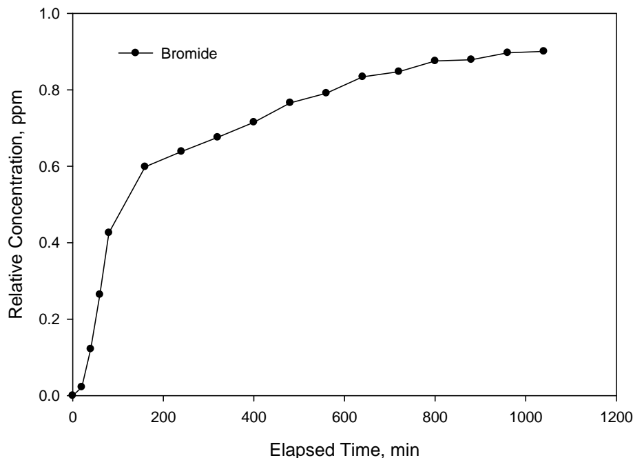
Figure 12. Bromide breakthrough curve for the AOC column containing 75% apatite, 20% organoclay (OCB -750), and 5% chitosan.
