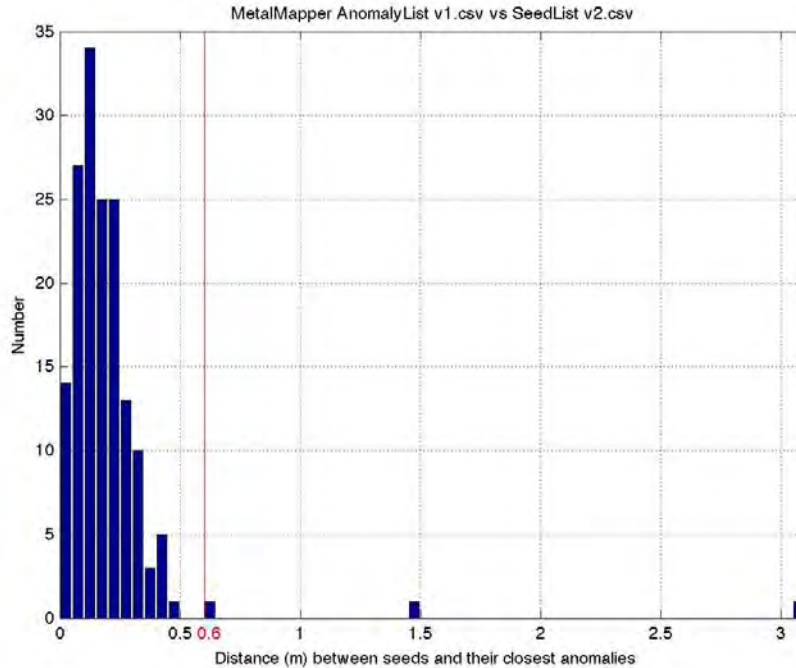
Figure 14: Distances between seeds and their closest MetalMapper anomalies. Three seeds were farther than 0.60 m (2 ft) from their closest anomaly.
