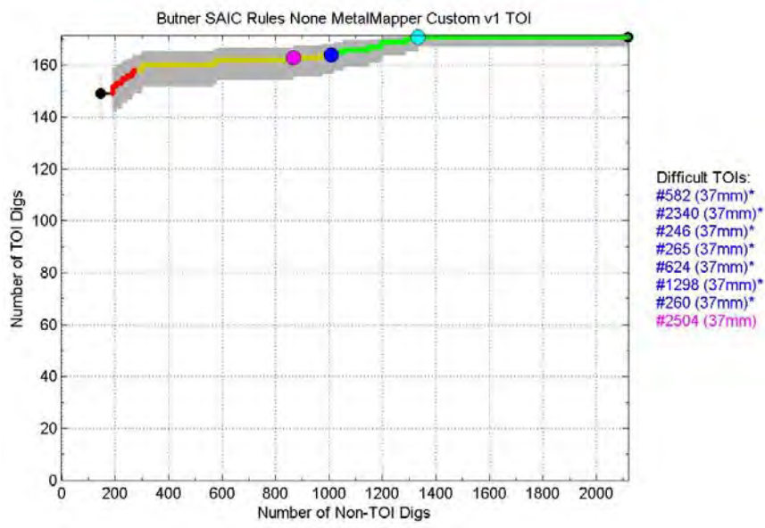
Figure 89: SAIC’s performance based on amplitudes, ratios, and decay rates of polarizabilities inverted from the MetalMapper static data using an IDL single-source dipole model and classified with a rules-based library matcher optimized over a custom training set. This second-pass custom training set was built from the “Likely TOI” anomalies in the previous figure. Identical to Figure 51 in the text.
