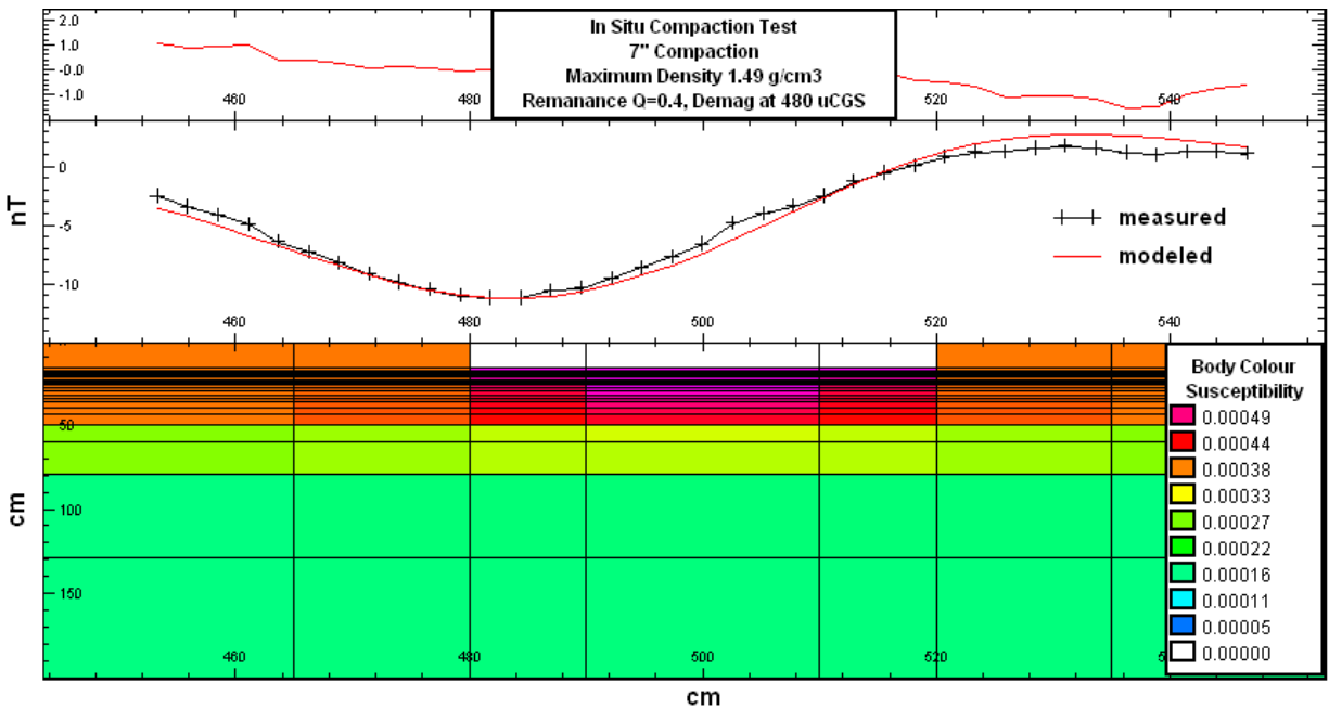
Figure 58. Forward Model of 18-cm Compaction Test
