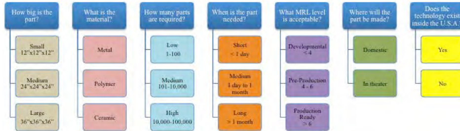
Figure 3. Decision Tree
