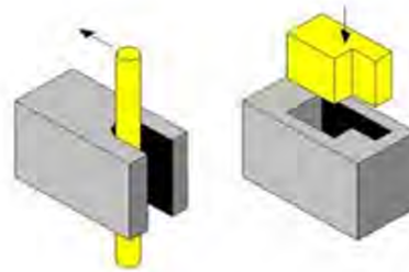
Wire and Ram type EDM
