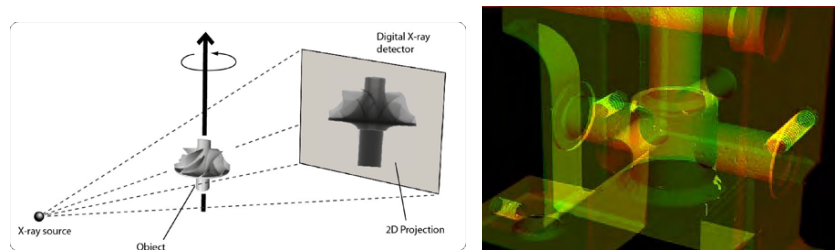
Figure 50. Schematic of Industrial Computed Tomography Technique (left) and Complex Object Imaged in this Way (right). (www.xviewct.com)
