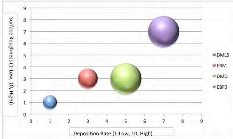
Figure 16. Comparison of Additive Beam Processes
