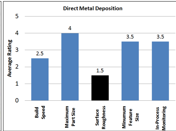
Figure 4a: Direct Metal Deposition
