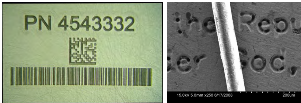
Figure 39. Marking ID Numbers via Laser Marking (left) or Micromachining (right). Fiber Shown in Right Hand Image for Scale is ~60 Microns Wide. Images Provided by MLPC, a Laser Processing Company. www.mlpc.com
