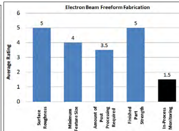
Figure 6a: Electron Beam Freeform Fabrication
