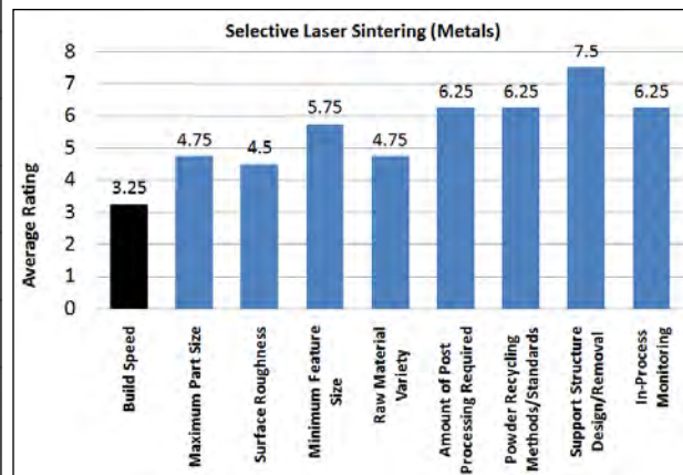
Figure 8a: Selective Laser Sintering (Metals)
