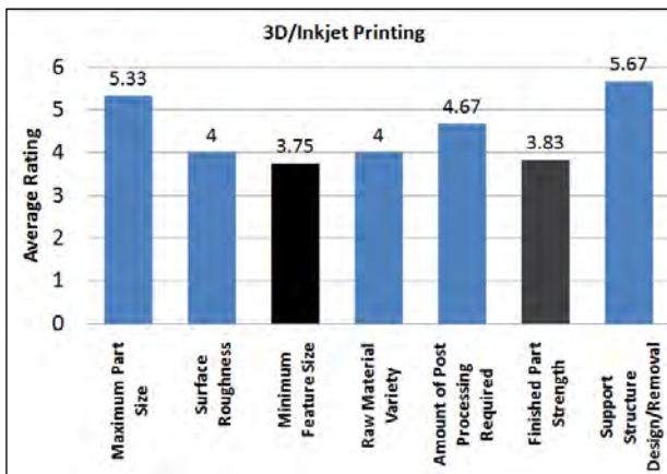
Figure 11a: 3D/Inkjet Printing
