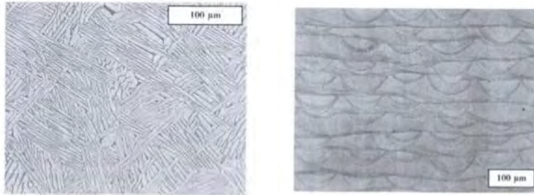
Figure 12. EBM Ti6Al4V Microstructure (left) versus DMLS CoCr Microstructure (right)
