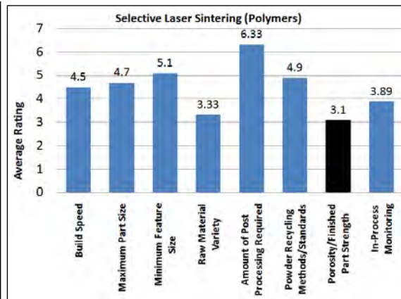
Figure 10a: Selective Laser Sintering (Polymers)
