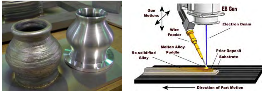
Figure 14. Pre/Post EBF3 Part (left) (nasa.gov), EBF3 Schematic (right) (sciaky.com)
