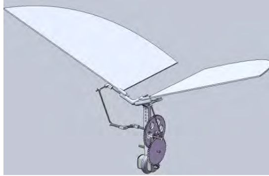
Figure 52. Example Assembly Design in Solidworks
