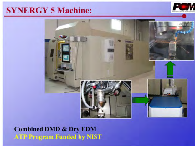
Figure 35. POM Hybrid DMD and Dry EDM Machine
