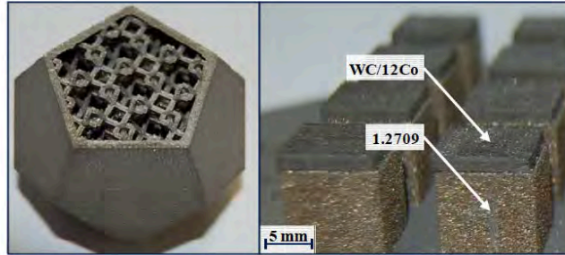
Fig. 1: Complex geometric parts produced by selective laser melting; a dodecahedron with internal structures (left) and a one dimensional multi-material structure (right)
