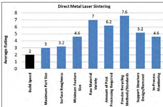
Figure 5a: Direct Metal Laser Sintering
