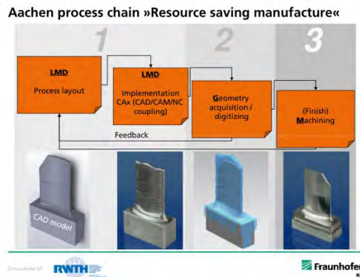
Figure 9. BLISK DMD Fabrication Process Developed by Fraunhofer
