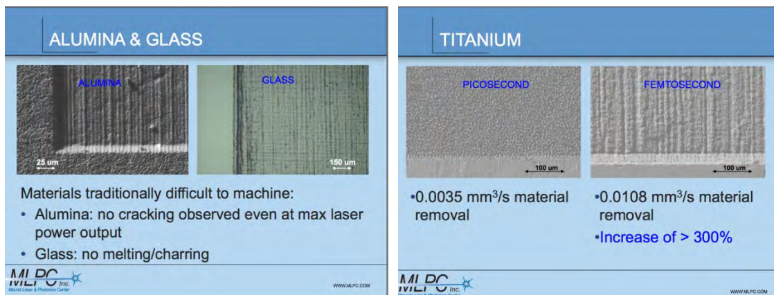
Figure 32. Femtosecond Laser Machining
