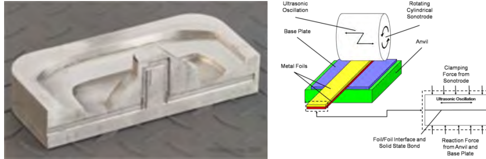
Figure 33. Ultrasonic Consolidation Example Part (left) and Schematic (right) www.solidica.com
