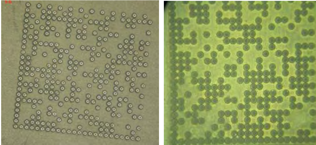
Figure 41. Examples of 2D Barcodes Marked by Dot Peening (left) and Laser Micromachining (right). Cells are 0.3 mm Wide
