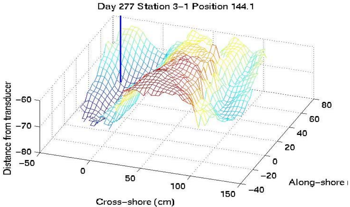
Figure 3. The local morphology measured by a scanning X/Y altimeter during the measurements shown in Figure 2. The location of the vertical acoustic doppler velocity profiles is shown as the vertical line near the cross-shore origin. The large amplitude, 1m scale ripples were typical of the
