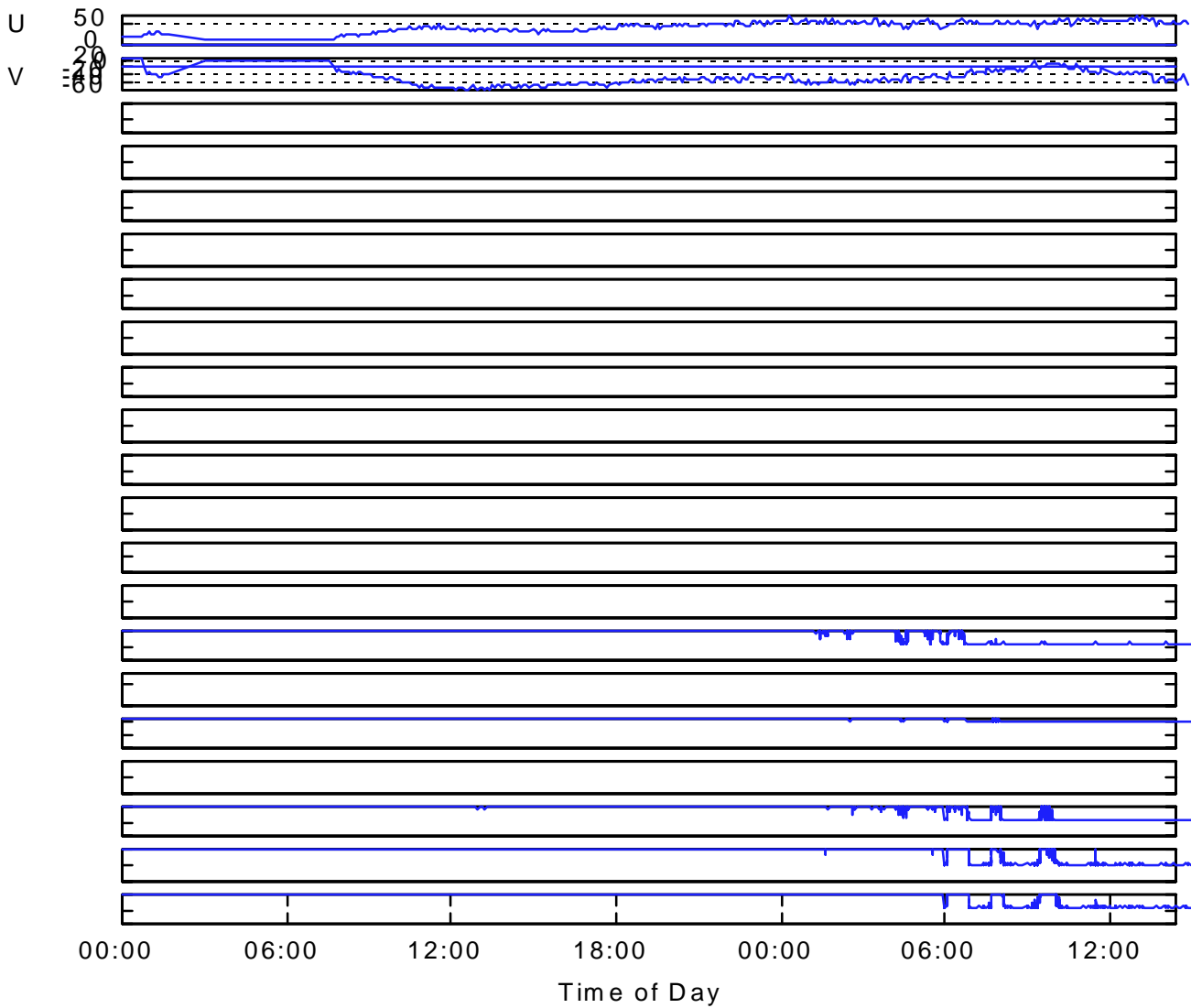
Figure 1: Time series of mean crossshore ( u ) and longshore ( v ) velocity and 19 channels of raw concentration measurements at site for the 19 th and 20 th of October 1997. FOBS is saturated when buried so bed level is near top of quiescent channels. Figure shows approximately 50 cm of erosion over a 36 hour period. Erosion starts off as a steady gradual lowering of the bed followed by a period of rapid bed oscillations.
