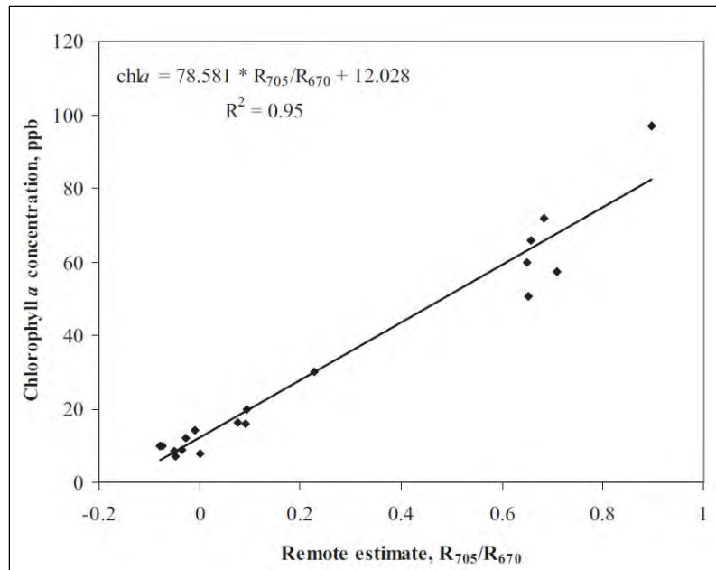
Figure 1. Example of a linear regression between laboratory-measured Chl concentrations in Lake Minnetonka, MN in 2005 with predicted Chl estimates using a common near infrared (NIR)/red band ratio (705/670 nm); the model illustrates strong correlation between measured and predicted estimations with high statistical significance, R^2 = 0.95 , which is a common measure of goodness of fit (Chipman et al. 2009).
