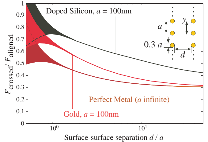
FIG. 2. (Color online) Ratio of the Casimir force between crossed wire arrays ( F_{\text{crossed}} ) over aligned wires [ F_{\text{aligned}}(y) ] between vacuum-separated nanowires of perfect metal, gold, and doped silicon (dopant density 10^{20}/\text{cm}^3 ). a \rightarrow \infty corresponds to using nondispersive \epsilon(i\xi \rightarrow 0) for all materials (because \xi is in units of c/a ). Shaded regions indicate the range of values that F_{\text{aligned}} takes over all relative lateral displacements y of the wire centers, with their higher (lower) boundary indicating the force for y = 0 ( y = a/2 ). PFA predicts, via Eq. (1), that the maximum of this ratio should exceed 1, which is only true for Si at d/a \sim 0.6 , and for gold/perfect metal at lower separations. Inset: details of the configuration examined.
