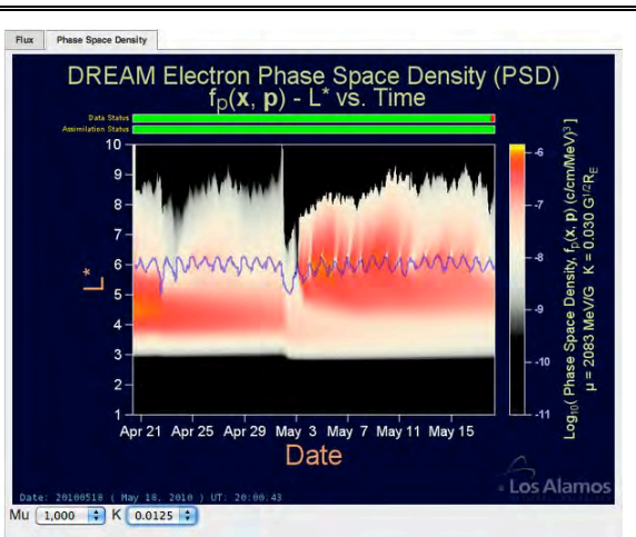
Figure 4: The actual assimilation in DREAM uses phase space density at fixed magnetic invariants ( \mu , K, L^* ). Assimilations are done for 25 different \mu -K pairs and are visible in the Phase Space Density tab.
