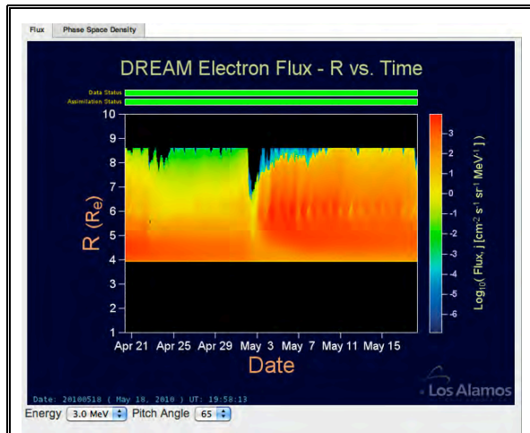
Figure 3: Final DREAM output is flux as a function of equatorial altitude (R) and time. Fluxes for 3 MeV and 65^\circ equatorial pitch angle are shown here but are selectable with the pull down menus just below the plot.
