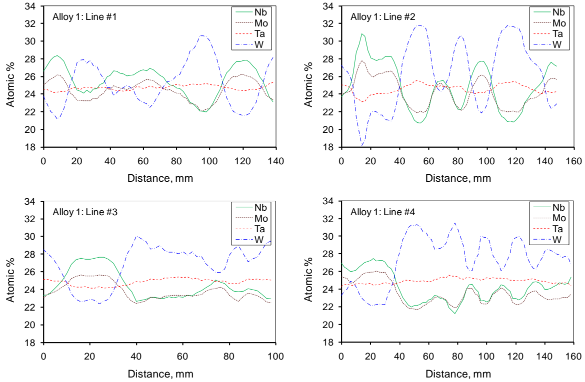
Figure 5. Distribution of elements in Alloy 1 along the lines shown in Figure 4 (a).
