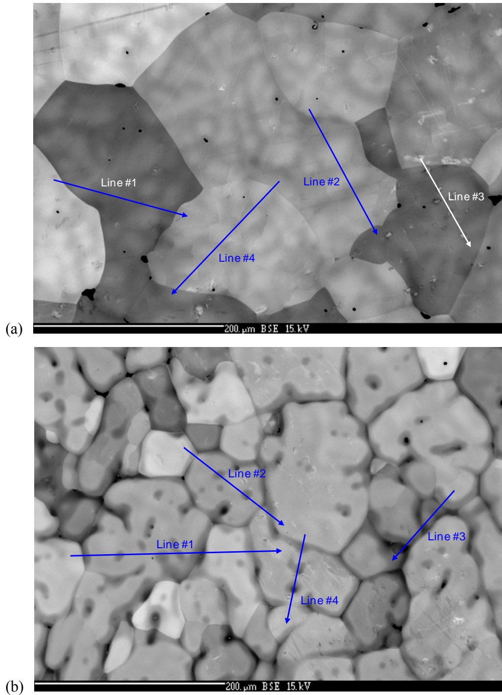
Figure 4. SEM backscatter electron images of the regions of (a) Alloy 1 and (b) Alloy 2 from which the EPMA analysis was conducted. The elemental composition gradients were determined along the drawn lines with the spacious resolution of 2 μm.
