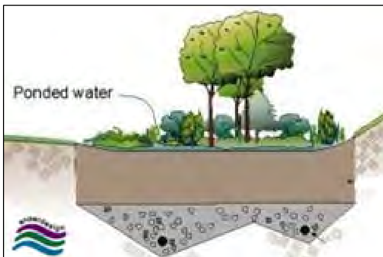
Figure 7. Bioretention system. 52
