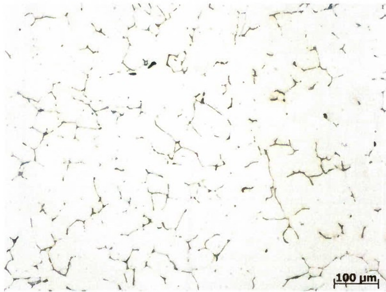
Figure 8 Micrograph of the 304 sample with no addition.
