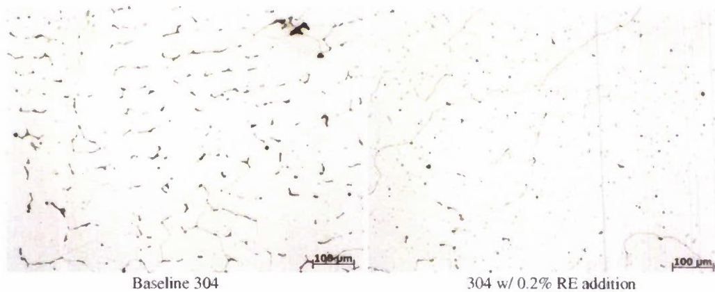
Figure 17 Typical micrographs from the rare earth addition experiments.
