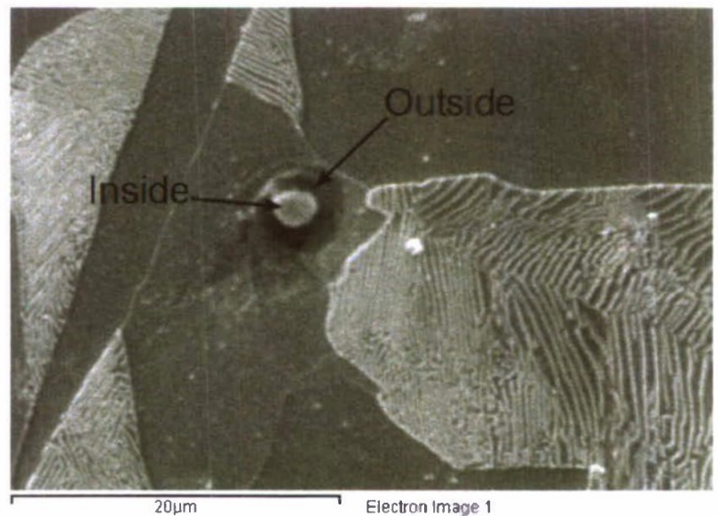
Figure 3 Typical RE inclusion from Test Casting 1
