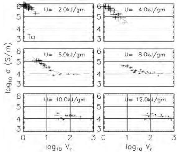
FIG. 9. Tantalum conductivity.
