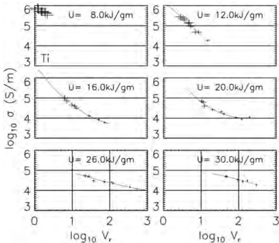
FIG. 8. Titanium conductivity. \times is from Ref. [13].
