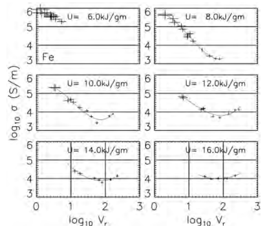
FIG. 5. Iron conductivity.
