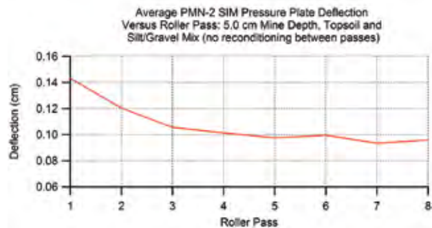
Image 11. Average pressure-plate deflection (cm) versus roller pass.
