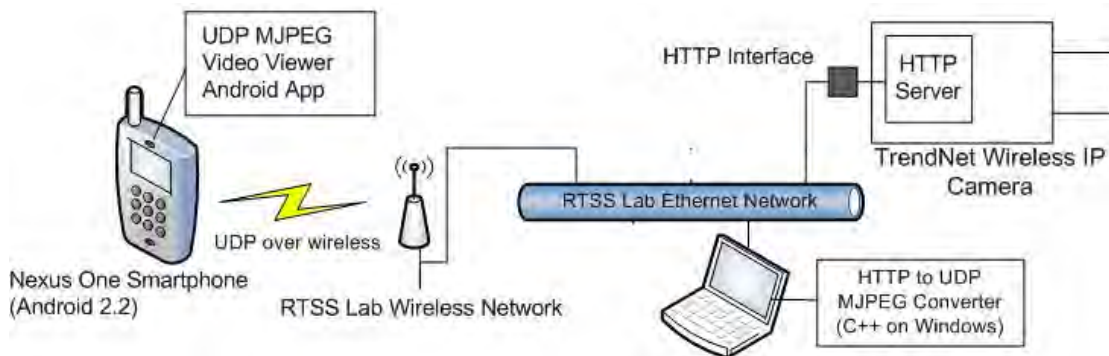
Figure 8-1: Use of UDP to Transport Video Frames
