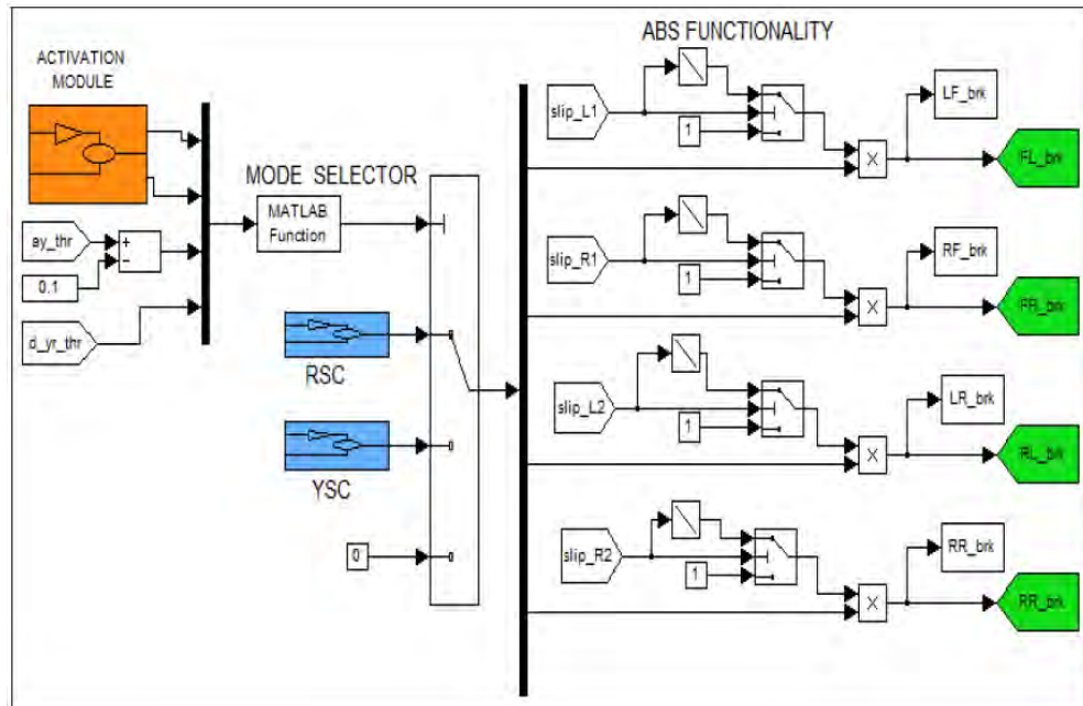
Figure 4-2: Sample Simulink Model for an ESC System [Kinjawadekar 2009]
