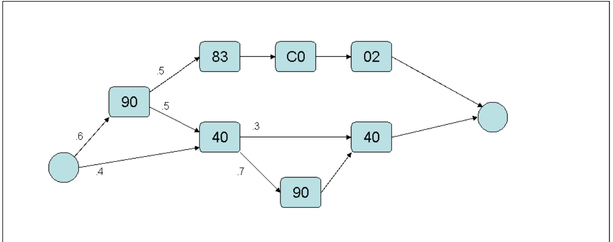
Figure 6-1: Simple HMM To Generate Behaviorally Equivalent Code Sequences
