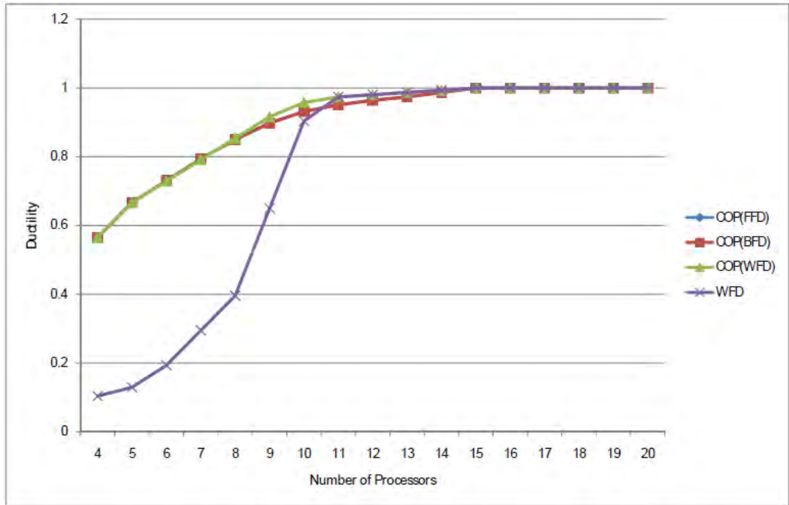
Figure 5-3: Ductility Evaluation
