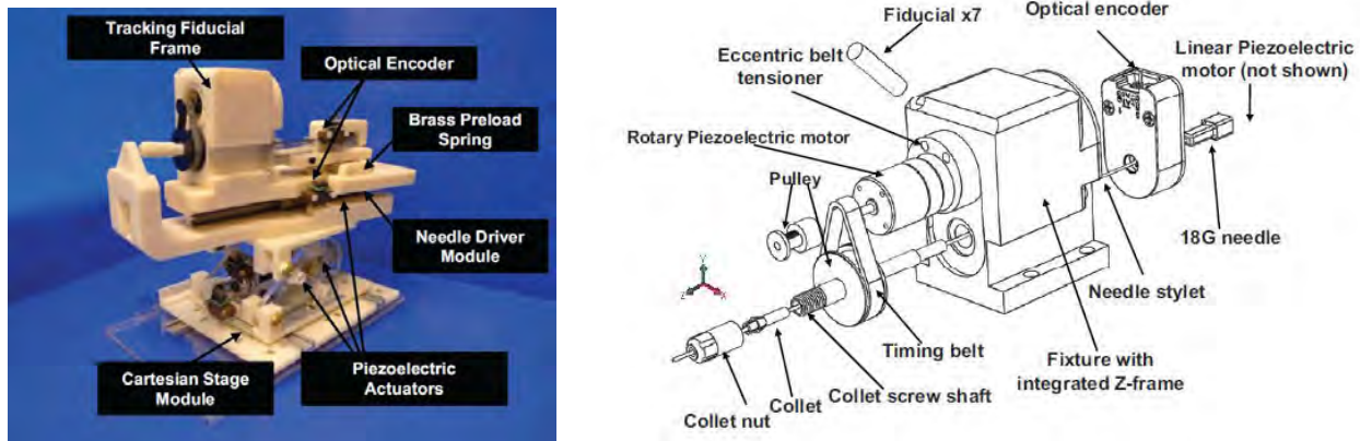
Figure 6 - Physical prototype of 6-DOF piezoelectric actuated needle placement robot (left). An exploded view of the needle clamping mechanism, fiducial frame and motor fixture (right).
