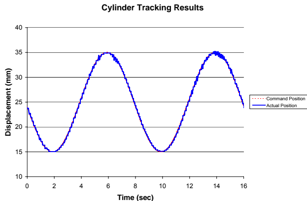
Fig. 13 Dynamic tracking results for the pneumatic cylinder for an 8sec period, 20mm amplitude sine wave.
