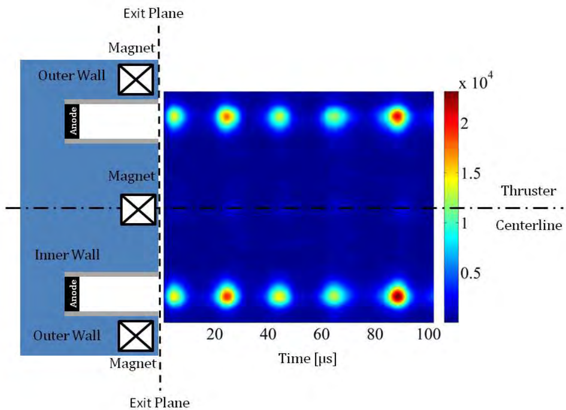
Figure 4.12: Plasma emission (arbitrary intensity) of BHT-600 as a function of space and time. Distance from the inner wall to the outer wall of the thruster was approximately 7.5 mm. Thruster was operating at nominal conditions. V_d = 300 V, I_d = 2.0 A, I_m = 1.75 A, \dot{m} = 2.6 mg/s of xenon.
