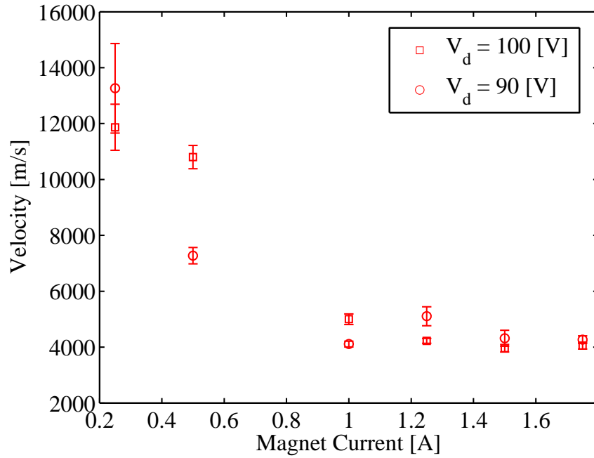
(a) Velocity of azimuthal plasma structures
