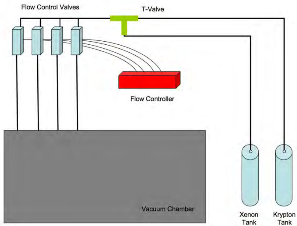
Figure 3.5: Propellant flow diagram for the Hall thrusters. Xenon and krypton propellant tanks are attached to a T-valve to allow the user to switch between either propellant while the vacuum chamber is pumped down. Four flow control valves, all controlled by the same flow controller, allow for precise flow rates to the anode and the cathode.
