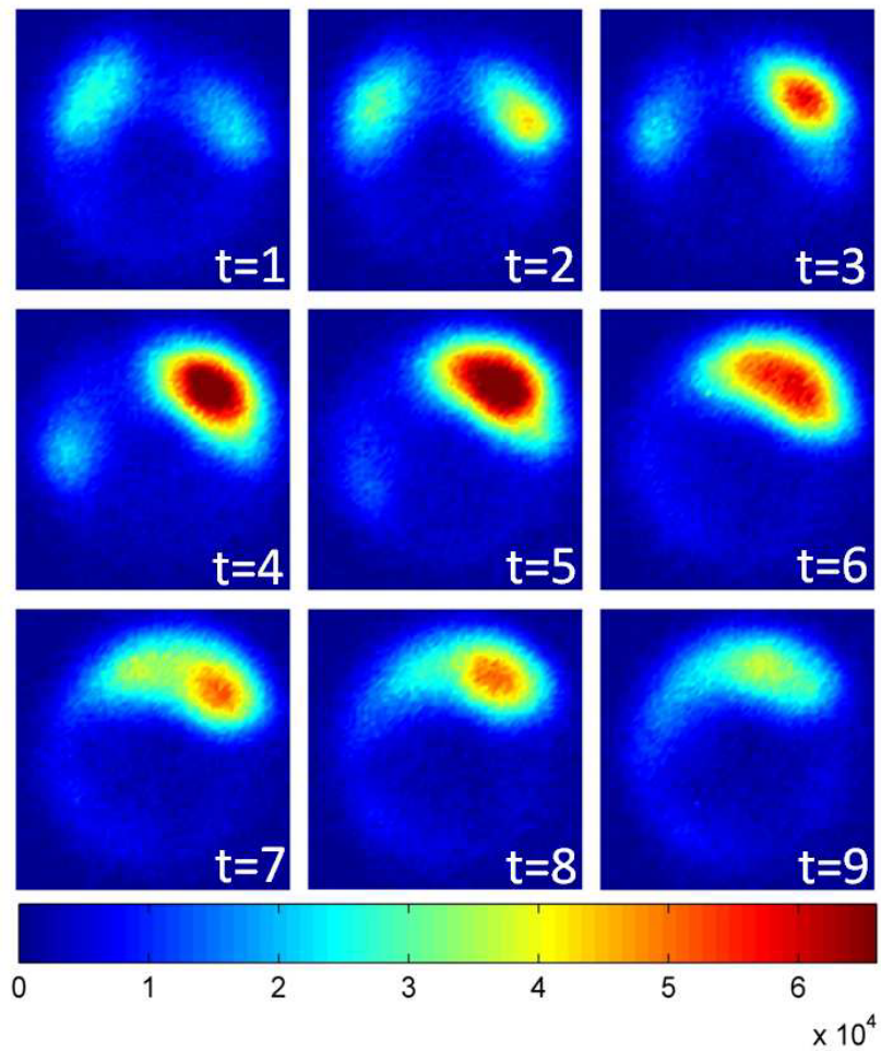
Figure 4.54: Sequential images (color enhanced) of BHT-200 azimuthal plasma structures. The two plasma structures were rotating in the E \times B direction about the center of the thruster where one plasma structure decreased in emission intensity while the other plasma structure simultaneously increased in intensity. Thruster was operating at off nominal conditions. V_d = 80 V, I_d = 0.8 A, I_m = 1.0 A, \dot{m} = 0.94 mg/s of xenon. The time between images was 1 \mu\text{s} with an exposure time of 750 ns. Arbitrary intensity.
